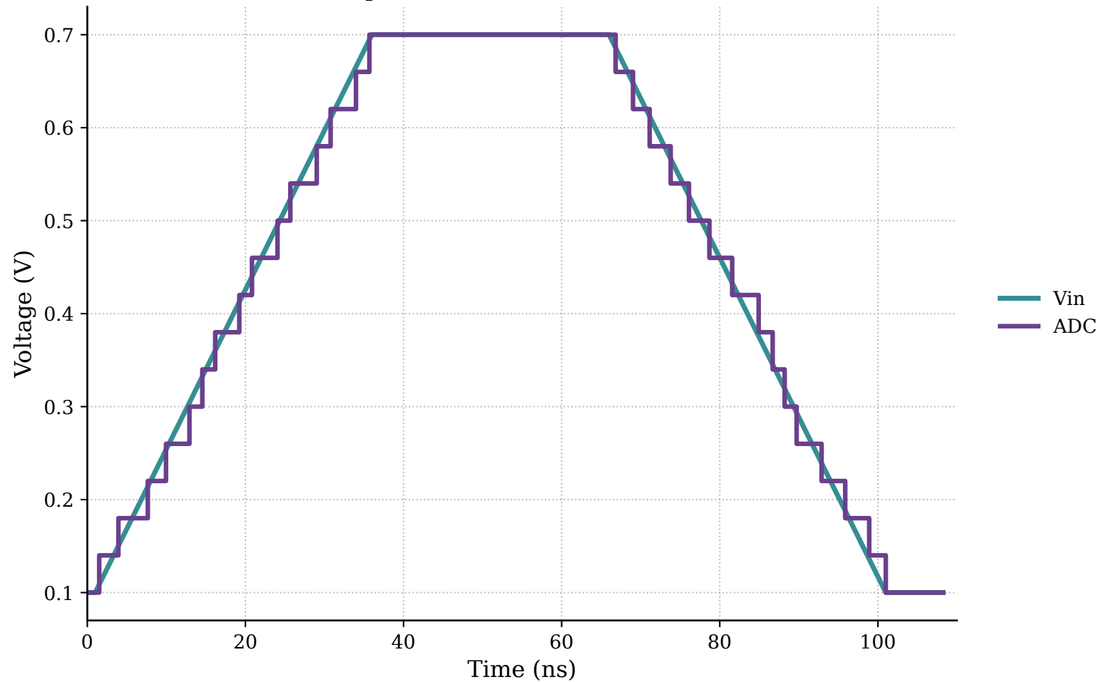
Input vs ADC Reconstruction
