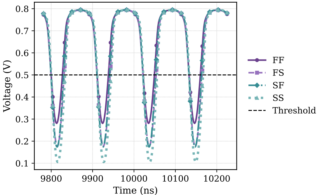
Corner Waveforms (Zoomed)
