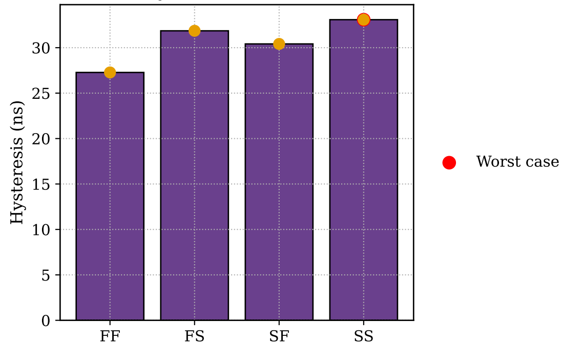
Hysteresis vs Corner
