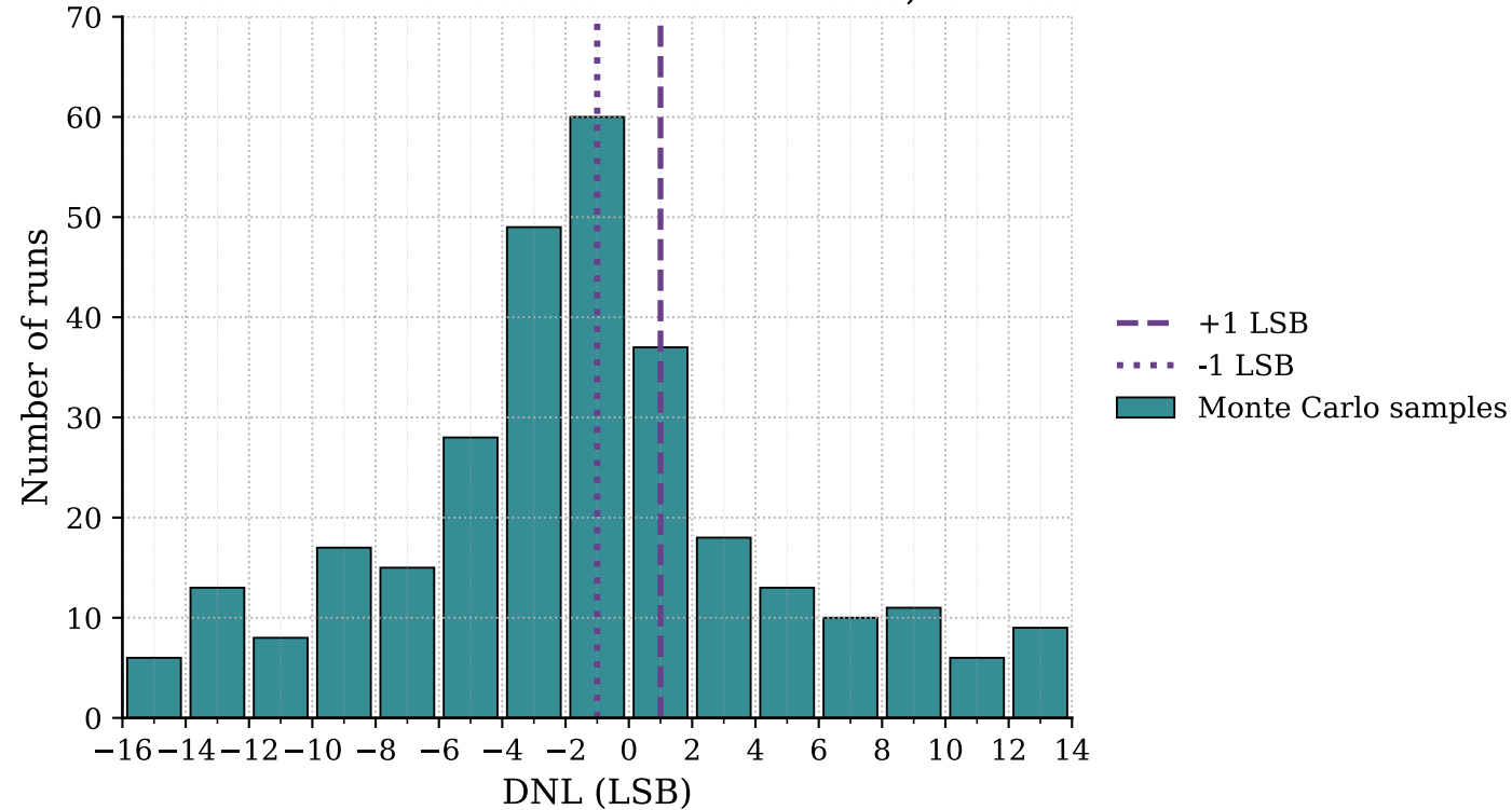
Monte Carlo: DNL between out1 and out0, N = 300
