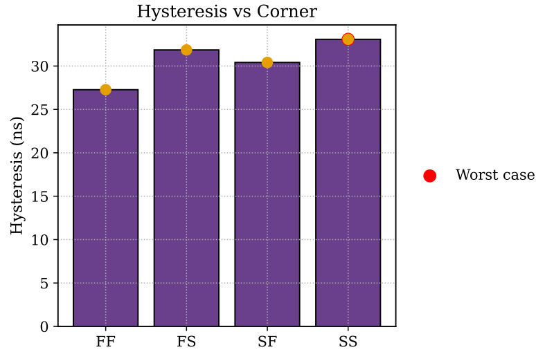
Figure 4.9: Input-referred hysteresis of the bulk-driven OTA follower at the four process corners, measured under the 9 MHz full-scale sinusoid, with the worst case marked at the slow SS corner.
