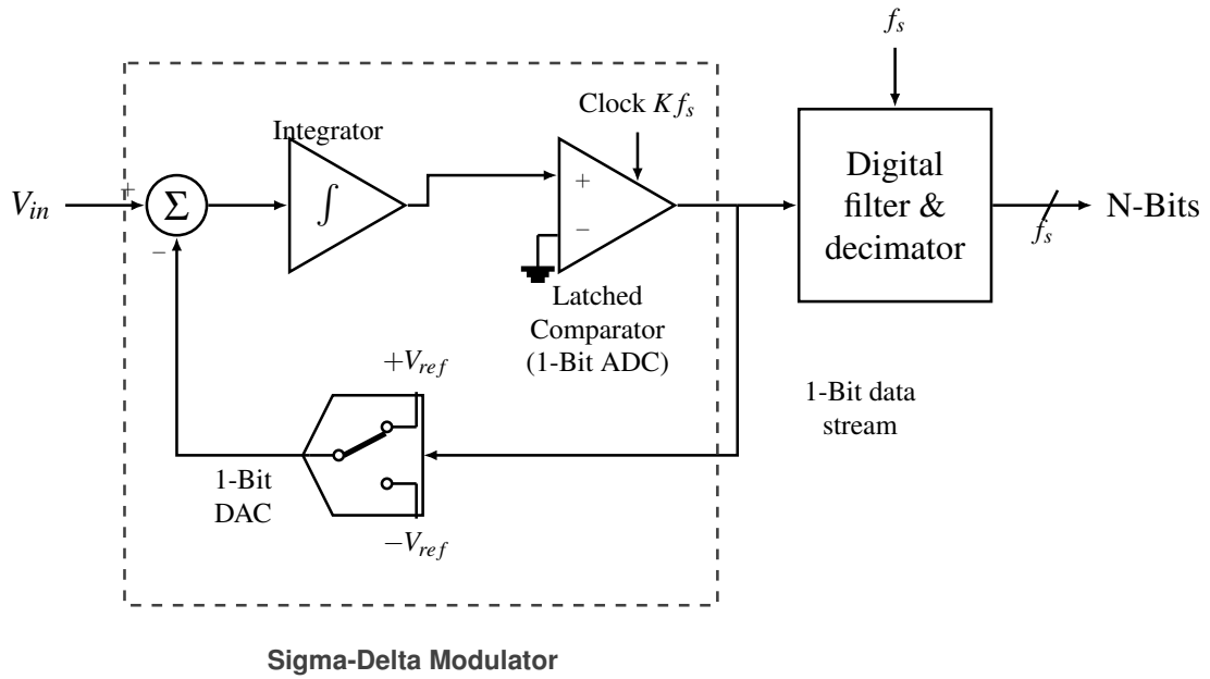
Figure 2.4: First-order sigma-delta ADC architecture illustrating the oversampling modulator with summer, integrator, 1-bit quantiser, feedback DAC, and digital decimation filter, which together implement noise shaping and high-resolution conversion [16, 120].
