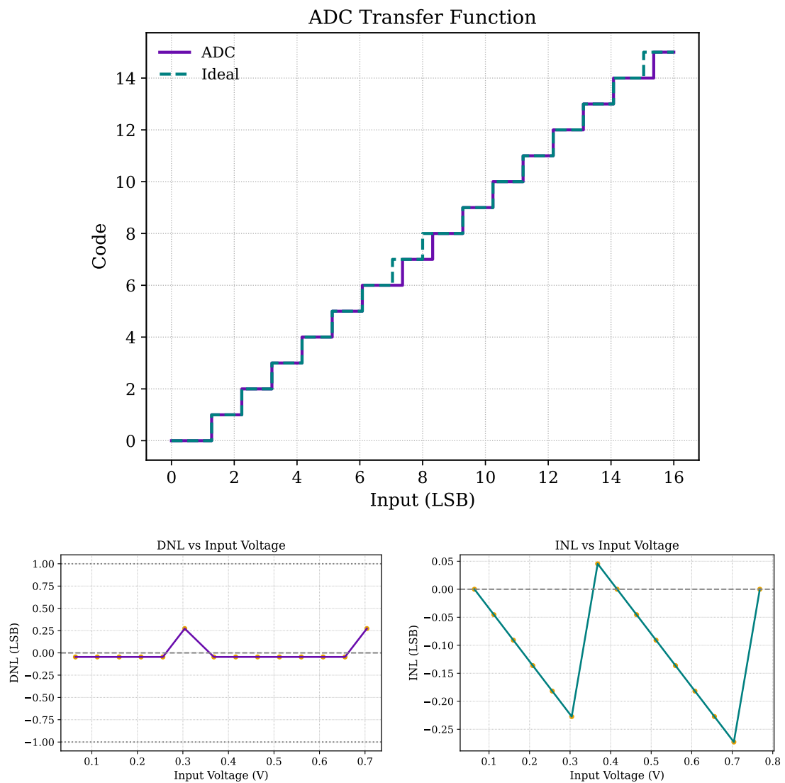
Figure 6.5: Static characterisation of the synchronous reference: (top) measured transfer function against the ideal staircase, (bottom left) DNL per code and (bottom right) INL per transition.
