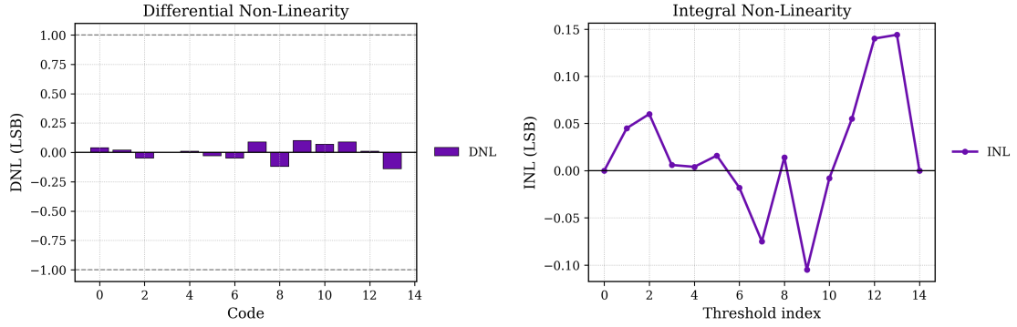
Figure 4.12: DNL per code (left) and INL per transition (right) of the final architecture at the typical (TT) corner.
