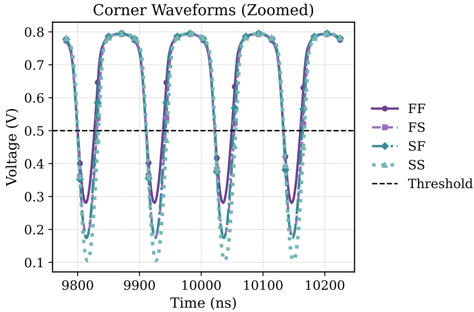
Figure 4.8: Response of the bulk-driven OTA follower across the four process corners (FF, FS, SF, SS). The output waveform diverges markedly between corners, most of all near the lower rail, the sensitivity that led to discarding the architecture.
