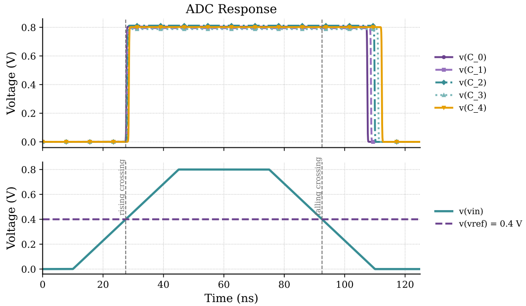
Figure 4.5: Simulated operation of the first architecture. The five comparator outputs (top) follow a trapezoidal input crossing the 0.4 V reference (bottom). The rising crossing is tracked sharply, but the falling transition lags well behind the input crossing, the slow-recovery asymmetry of the high-impedance current-mirror node.
