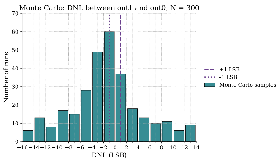
Figure 6.3: Monte Carlo distribution of the DNL of the code between two adjacent slicers ( \text{out}_0 and \text{out}_1 ), with the \pm 1 LSB limits marked.
