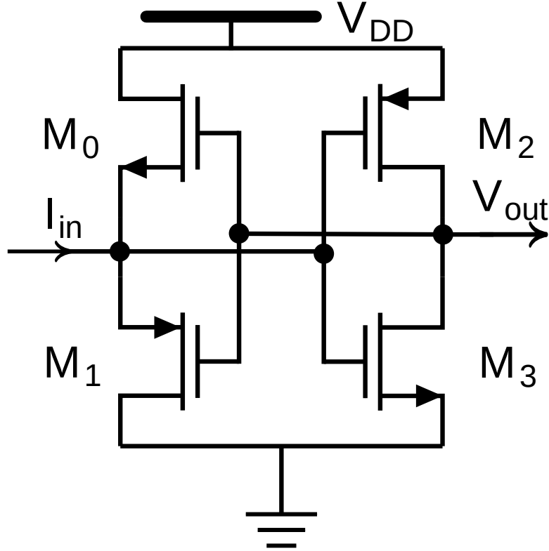
Figure 2.7: Transistor-level schematic of the Traff current comparator.
