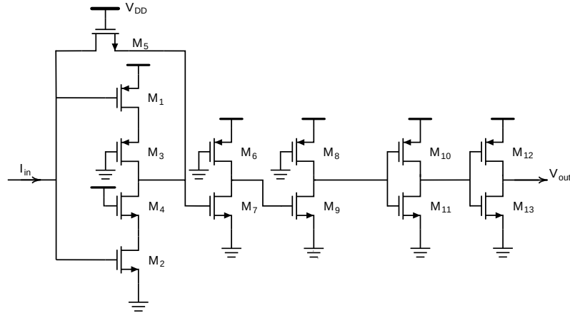
Figure 2.8: Transistor-level schematic of the Lu Chen current comparator.
