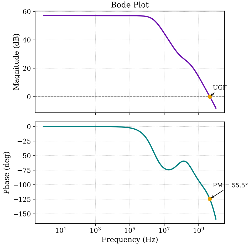
Figure 4.11: Open-loop magnitude and phase response of the complementary five-transistor OTA, showing the single dominant pole and the wide phase margin.
