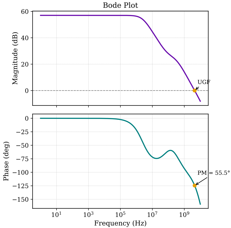
Figure 3.9: Open-loop magnitude and phase response of the complementary five-transistor OTA, showing the single dominant pole and the wide phase margin.
