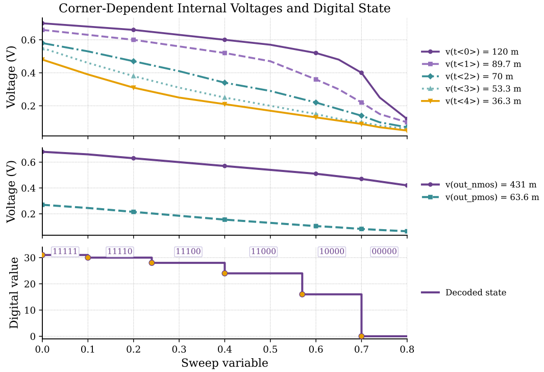
Figure 3.5: Simulated DC response of the second-architecture stage. The complementary outputs (out_nmos, out_pmos) and the internal node voltages never reach the supply rails and the transfer is visibly non-linear, the headroom shortfall predicted by equation (3.9) at the 0.8 V supply.
