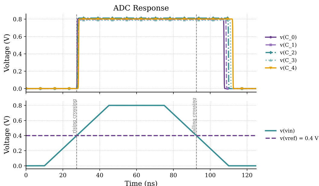
Figure 3.3: Simulated operation of the first architecture. The five comparator outputs (top) follow a trapezoidal input crossing the 0.4 V reference (bottom). The rising crossing is tracked sharply, but the falling transition lags well behind the input crossing, the slow-recovery asymmetry of the high-impedance current-mirror node.
