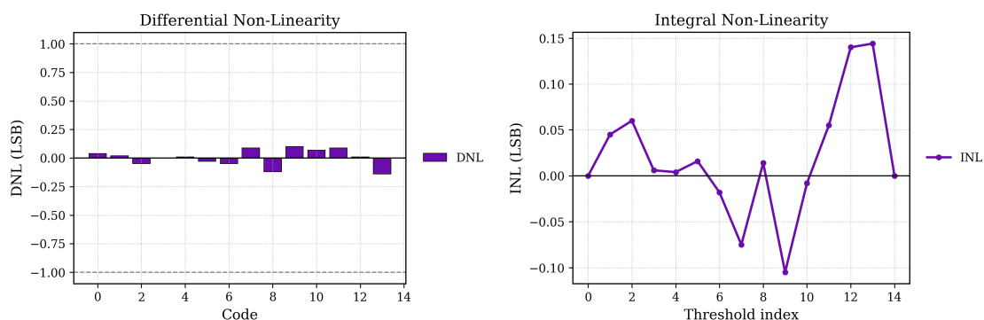
Figure 3.10: DNL per code (left) and INL per transition (right) of the final architecture at the typical (TT) corner.
