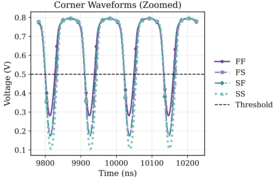
Figure 3.6: Response of the bulk-driven OTA follower across the four process corners (FF, FS, SF, SS). The output waveform diverges markedly between corners, most of all near the lower rail, the sensitivity that led to discarding the architecture.
