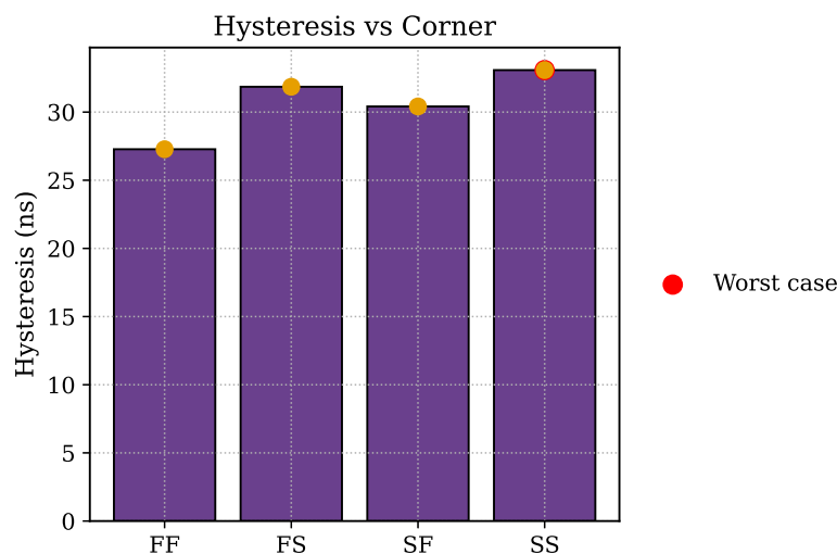
Figure 3.7: Input-referred hysteresis of the bulk-driven OTA follower at the four process corners, measured under the 9 MHz full-scale sinusoid, with the worst case marked at the slow SS corner.
