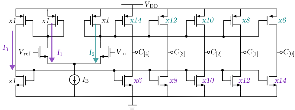
Figure 3.2: Transistor-level schematic of the first architecture, the current-mirror Flash ADC, showing the differential input pair driven by V_{ref} and V_{in} , the tail current source I_B and the five current-mirror output branches whose PMOS and NMOS width ratios set the thermometer thresholds C[4] down to C[0] .
