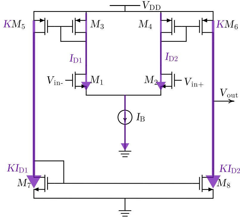
Figure 3.1: Transconductance cell of the current-mirror Flash ADC at equilibrium, showing the differential pair M_1, M_2 , the mirror loads M_3, M_4 and the K -scaled output copies KI_{D1}, KI_{D2} .
