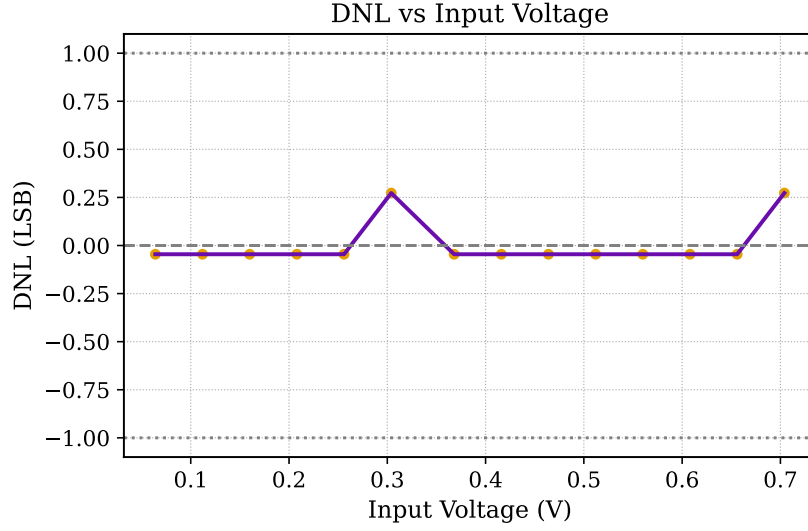
Figure 4.8: DNL per code of the synchronous reference.
