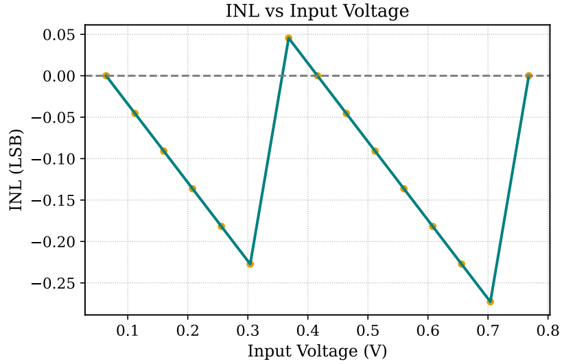
Figure 4.9: INL per transition of the synchronous reference.
