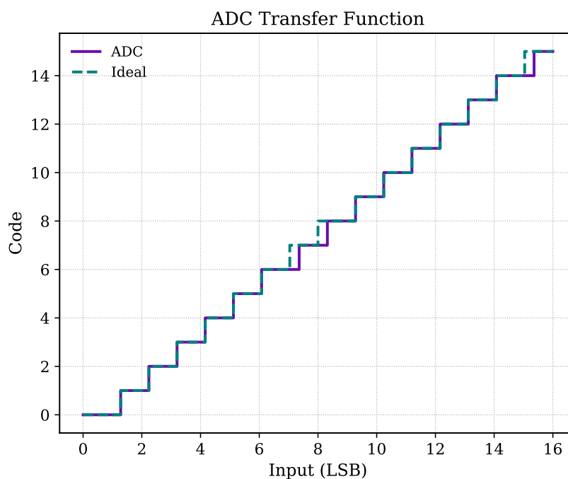
Figure 4.7: Simulated transfer function of the synchronous reference against the ideal staircase.
