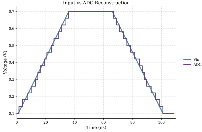
Figure 4.2: Trapezoidal pulse input ( V_{in} ) and reconstructed converter output (ADC) during the static-linearity test.
