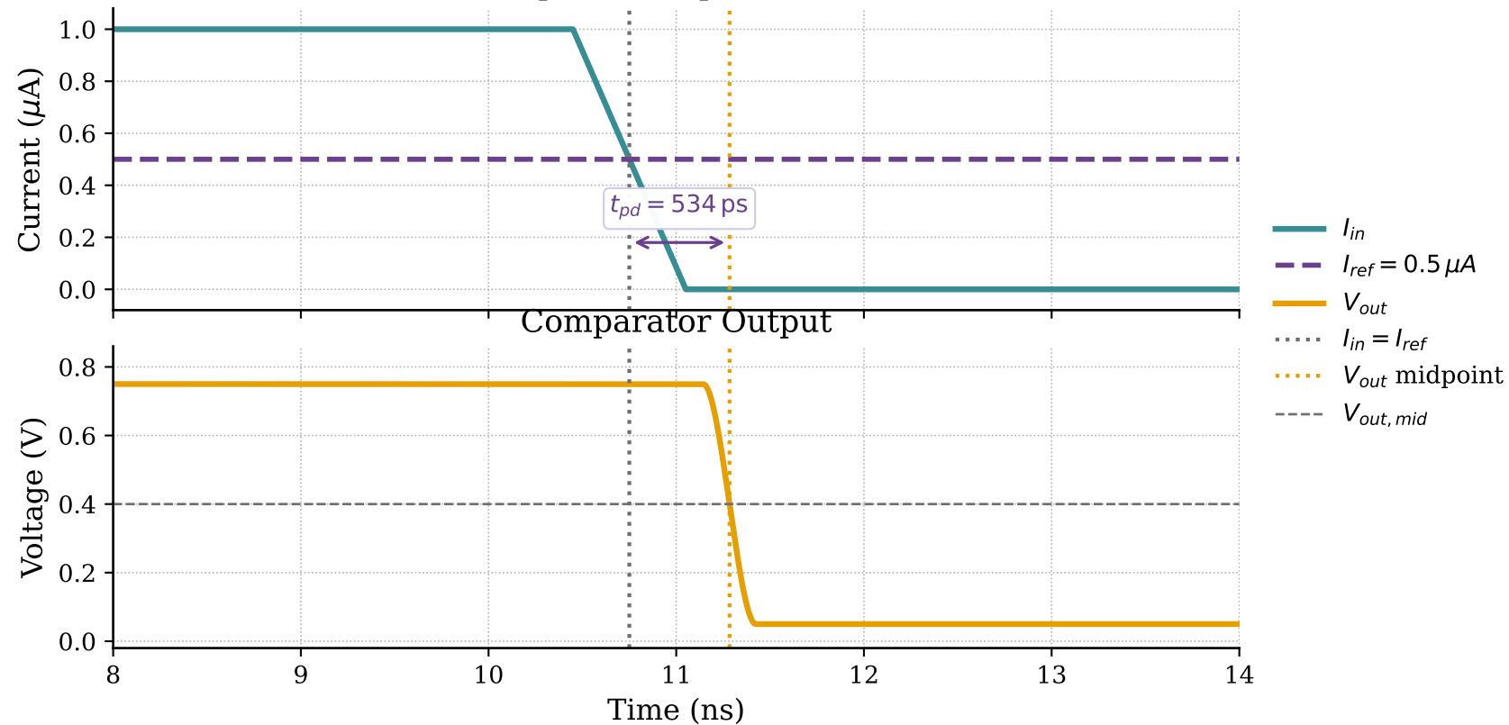
Comparator Input Current
