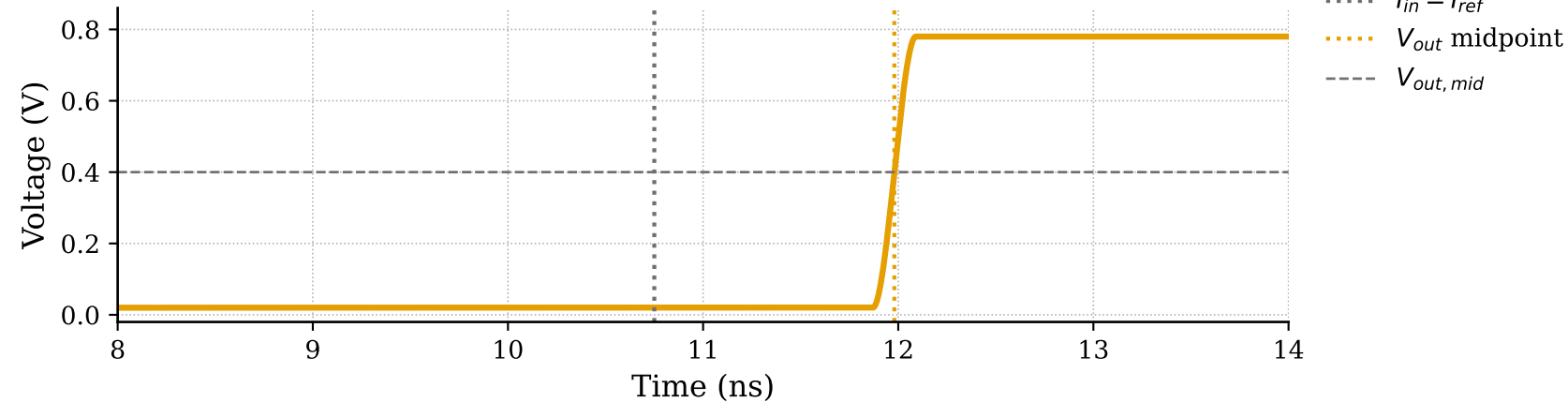
Comparator Output
