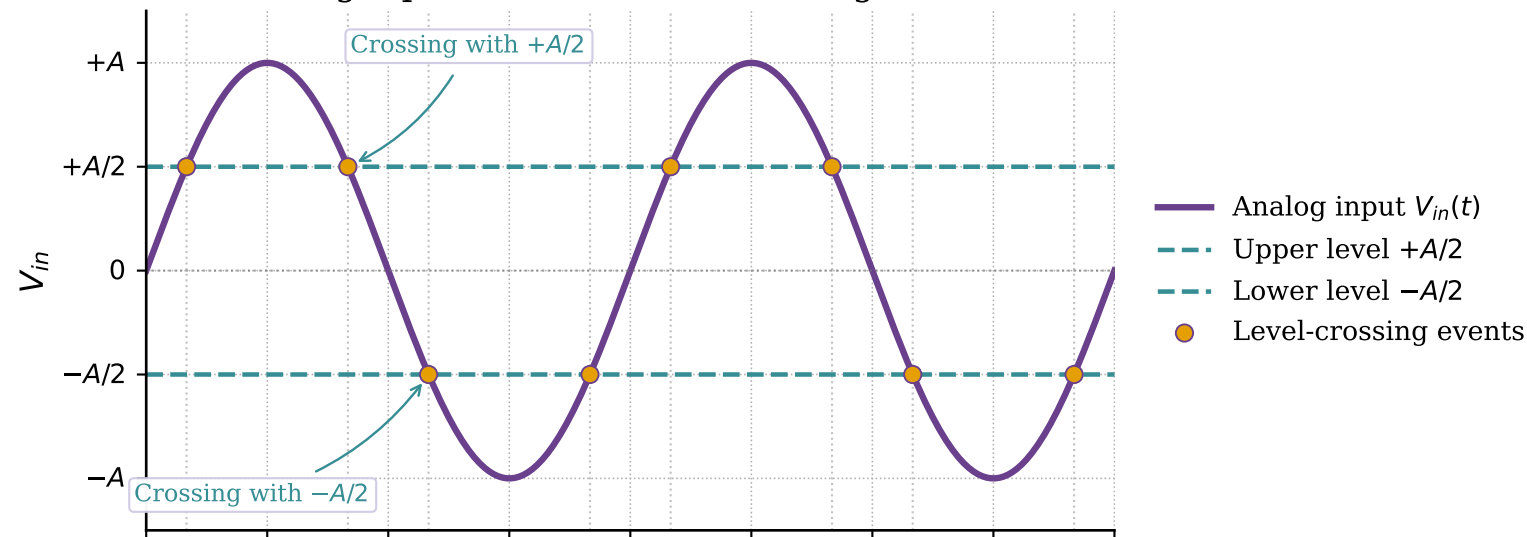
Analog input and threshold-crossing instants
