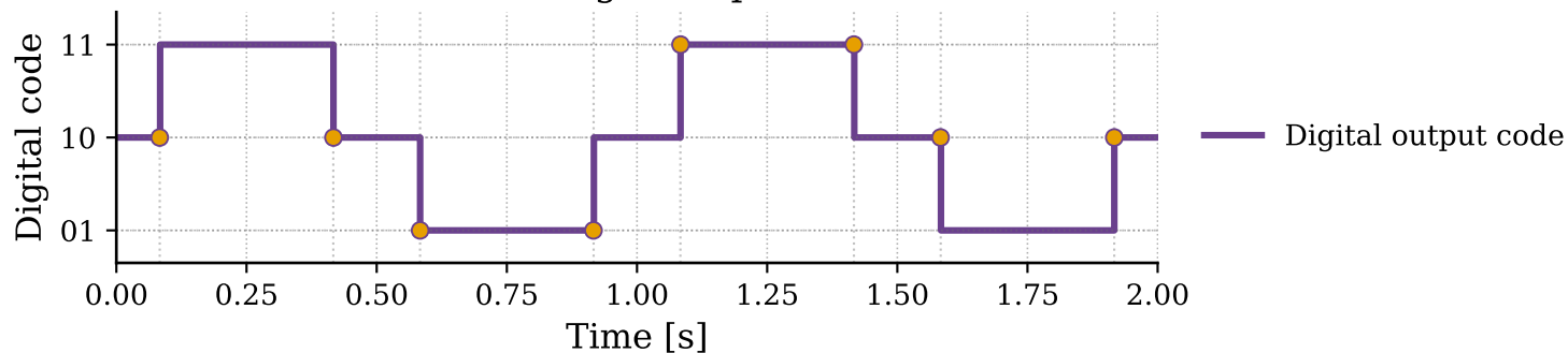
Event-driven digital representation
