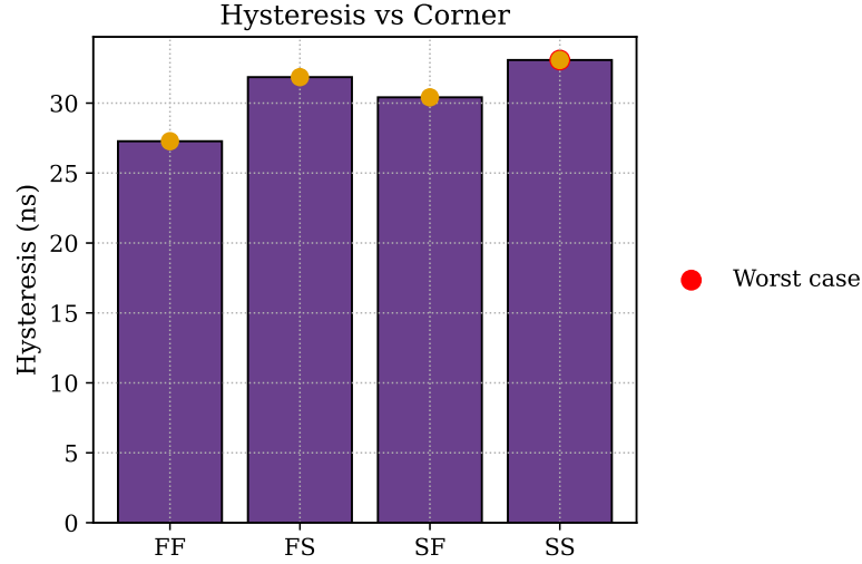
Figure 3.10: Input-referred hysteresis of the bulk-driven OTA follower at the four process corners, measured under the 9 MHz full-scale sinusoid, with the worst case marked at the slow SS corner.
