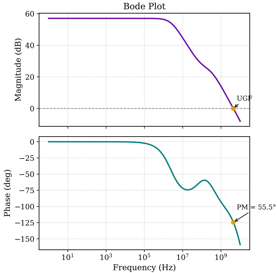
Figure 3.12: Open-loop magnitude and phase response of the complementary five-transistor OTA, showing the single dominant pole and the wide phase margin.
