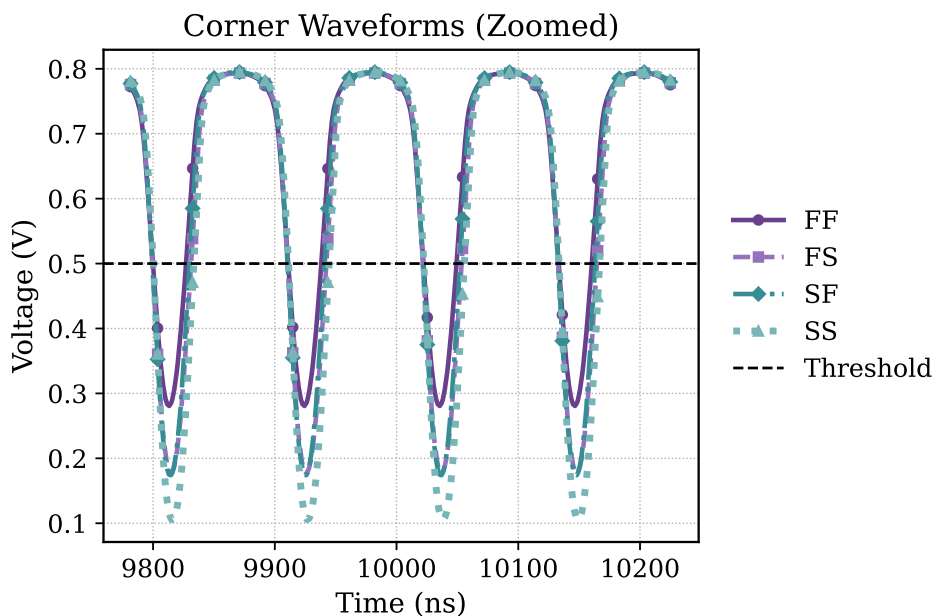
Figure 3.9: Response of the bulk-driven OTA follower across the four process corners (FF, FS, SF, SS). The output waveform diverges markedly between corners, most of all near the lower rail, the sensitivity that led to discarding the architecture.
