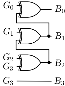
Figure 2.9: Gray-to-binary conversion logic of the synchronous reference encoder.
