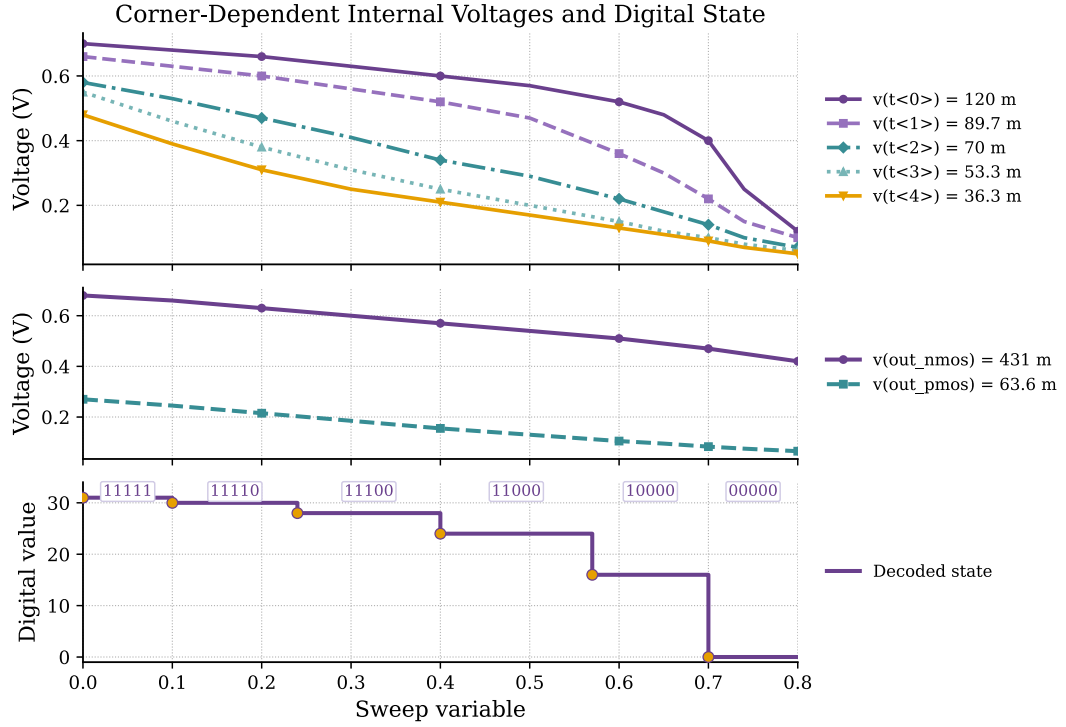
Figure 3.7: Simulated DC response of the second-architecture stage. The complementary outputs (out_nmos, out_pmos) and the internal node voltages never reach the supply rails and the transfer is visibly non-linear, the headroom shortfall predicted by equation (3.8) at the 0.8 V supply.
