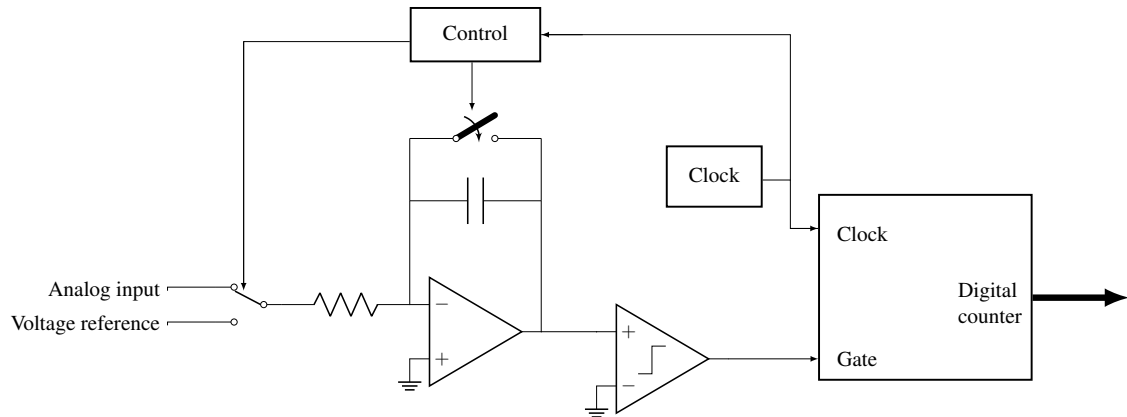
Figure 2.5: Dual-slope (integrating) ADC architecture showing the charging phase where an unknown input signal is integrated for a fixed time, and the discharge phase where a precise reference voltage drives the capacitor back to zero. The conversion time is proportional to the input voltage, providing excellent accuracy and noise rejection at the expense of low throughput.
