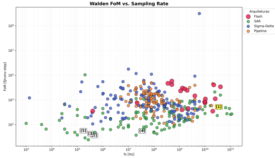
Figure 2.9: Walden FoM vs. Sampling Frequency (Flash reference [1] highlighted)
