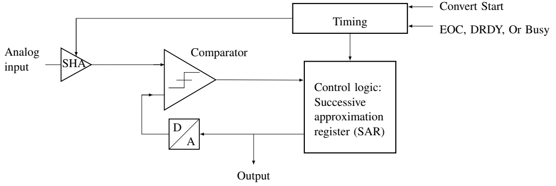
Figure 2.2: Successive Approximation Register (SAR) ADC architecture showing the sample-and-hold amplifier (SHA), comparator, digital-to-analog converter (DAC), and control logic. The SAR logic iteratively approximates the input signal by testing each bit from MSB to LSB, achieving high energy efficiency at moderate speeds [110].
