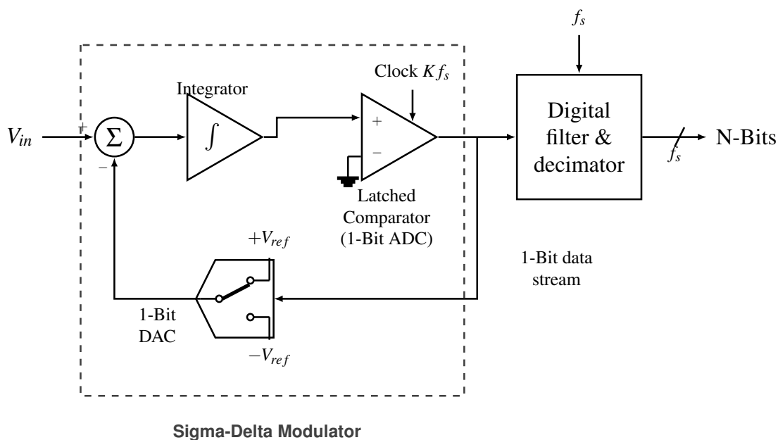
Figure 2.4: First-order sigma-delta ADC architecture illustrating the oversampling modulator with summer, integrator, 1-bit quantiser, feedback DAC, and digital decimation filter, which together implement noise shaping and high-resolution conversion [15, 119].
