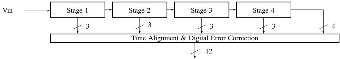
Figure 2.3: Pipeline ADC architecture showing multiple conversion stages operating in parallel on different input samples. Each stage resolves a subset of bits, generates a partial digital output, and amplifies the residue for the next stage. The pipelined structure enables high-throughput operation at the expense of increased latency and circuit complexity.
