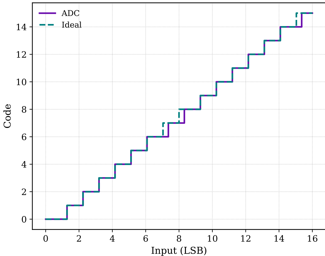
ADC Transfer Function
