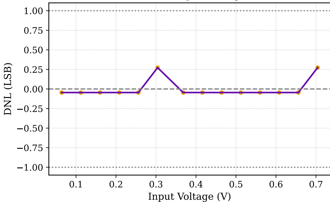
DNL vs Input Voltage
