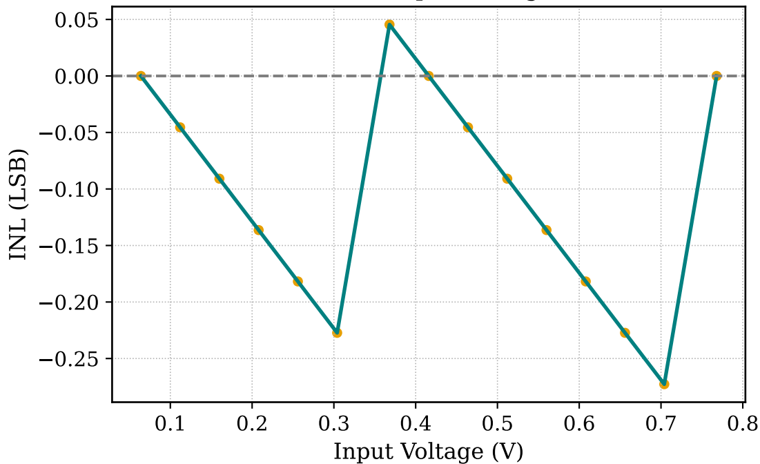
INL vs Input Voltage
