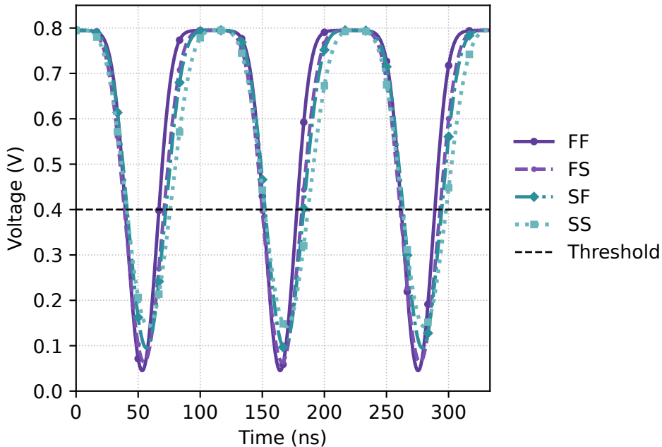
Corner Waveforms
