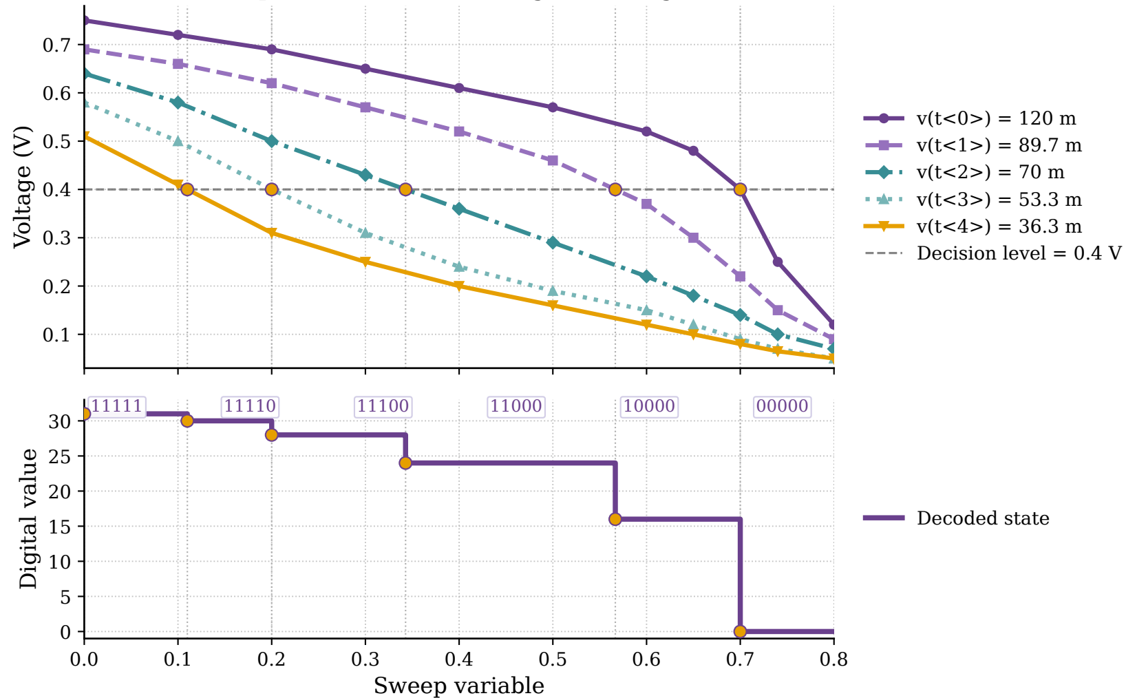
Corner-Dependent Internal Voltages and Digital State
