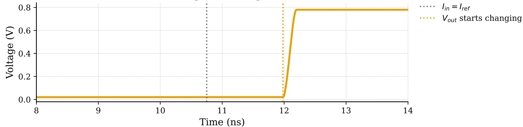
Comparator Output
