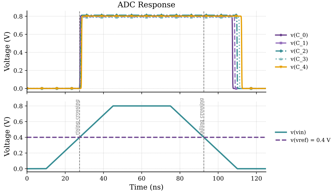
Figure 3.4: Simulated operation of the first architecture. The five comparator outputs (top) follow a trapezoidal input crossing the 0.4 V reference (bottom). The rising crossing is tracked sharply, but the falling transition lags well behind the input crossing, the slow-recovery asymmetry of the high-impedance current-mirror node.
