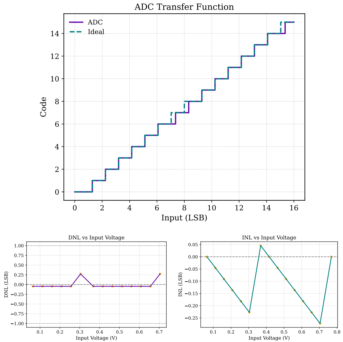
Figure 4.4: Static characterisation of the synchronous reference: (top) measured transfer function against the ideal staircase, (bottom left) DNL per code and (bottom right) INL per transition.
