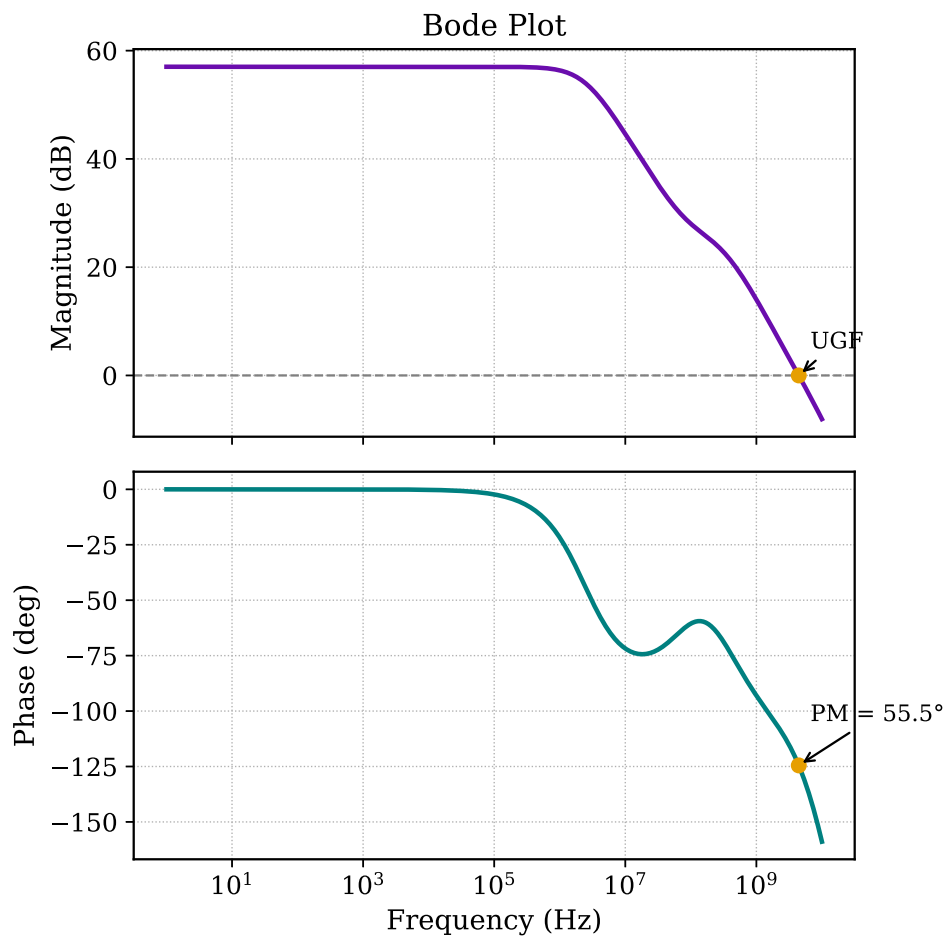
Figure 3.10: Open-loop magnitude and phase response of the complementary five-transistor OTA, showing the single dominant pole and the wide phase margin.
