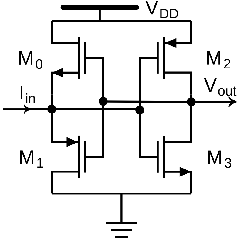
Figure 2.6: Transistor-level schematic of the Traff current comparator.
