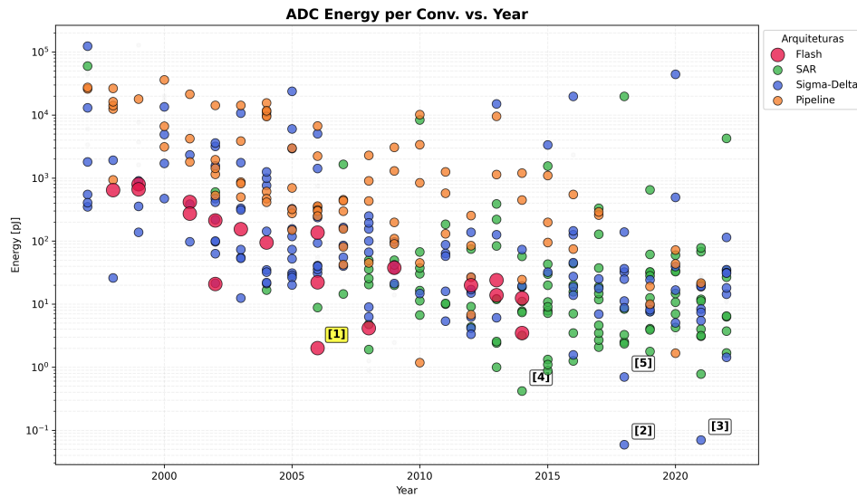
Figure 2.14: Energy per Conversion vs. Year (Flash reference [1] highlighted)
