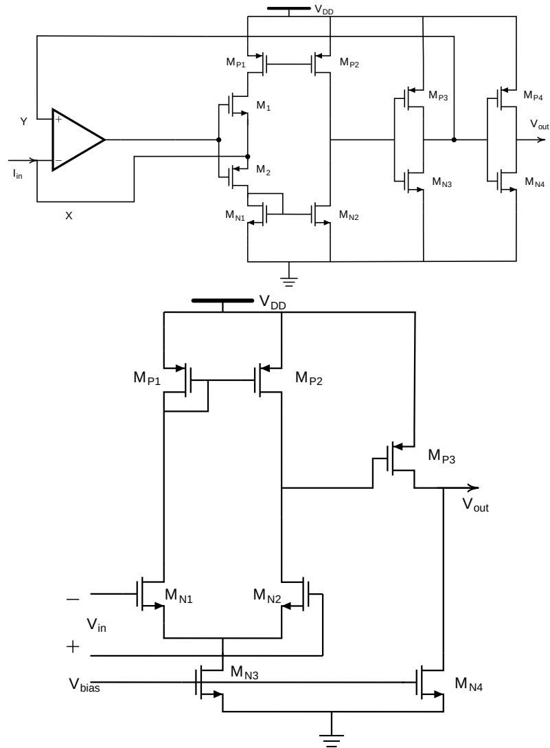
Figure 2.10: Transistor-level schematic of the CC-II-based current comparator, with its internal operational amplifier subcircuit shown below.
