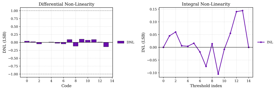
Figure 3.11: DNL per code (left) and INL per transition (right) of the final architecture at the typical (TT) corner.
