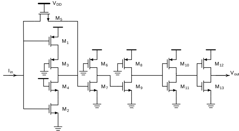
Figure 2.7: Transistor-level schematic of the Lu Chen current comparator.
