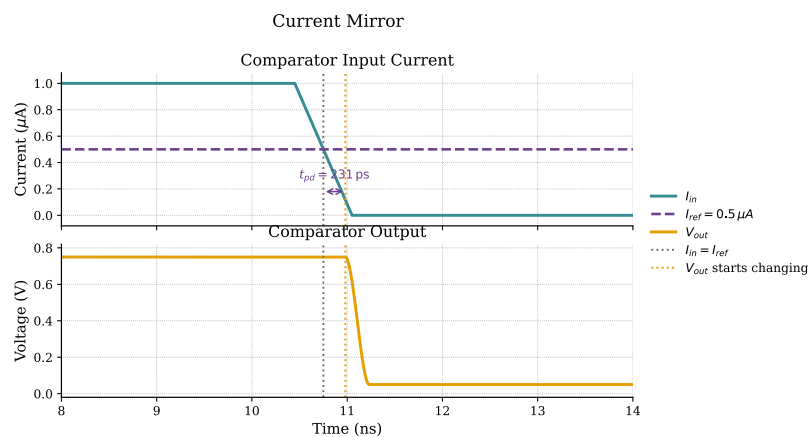
(a) Current-mirror
