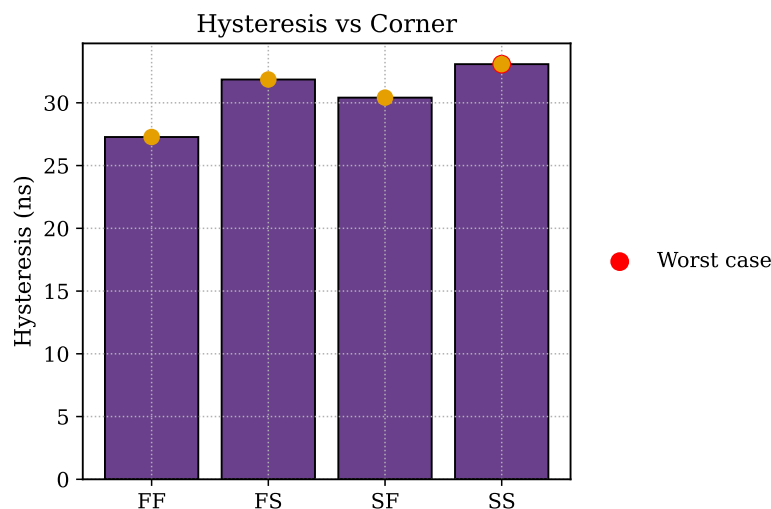
Figure 3.8: Input-referred hysteresis of the bulk-driven OTA follower at the four process corners, measured under the 9 MHz full-scale sinusoid, with the worst case marked at the slow SS corner.
