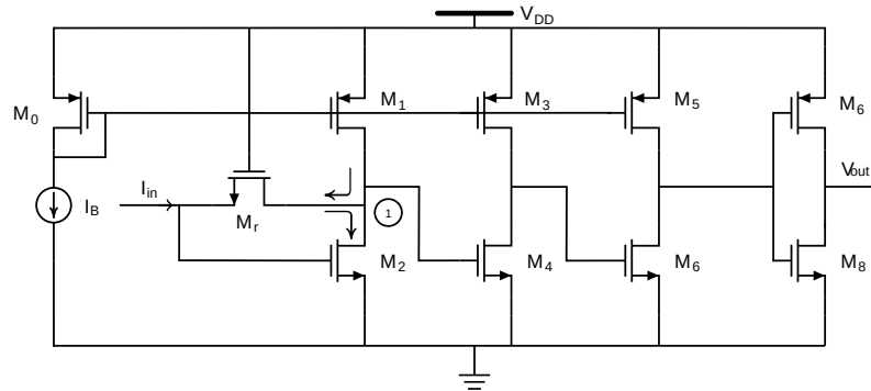
Figure 2.9: Transistor-level schematic of the Min and Kim current comparator.
