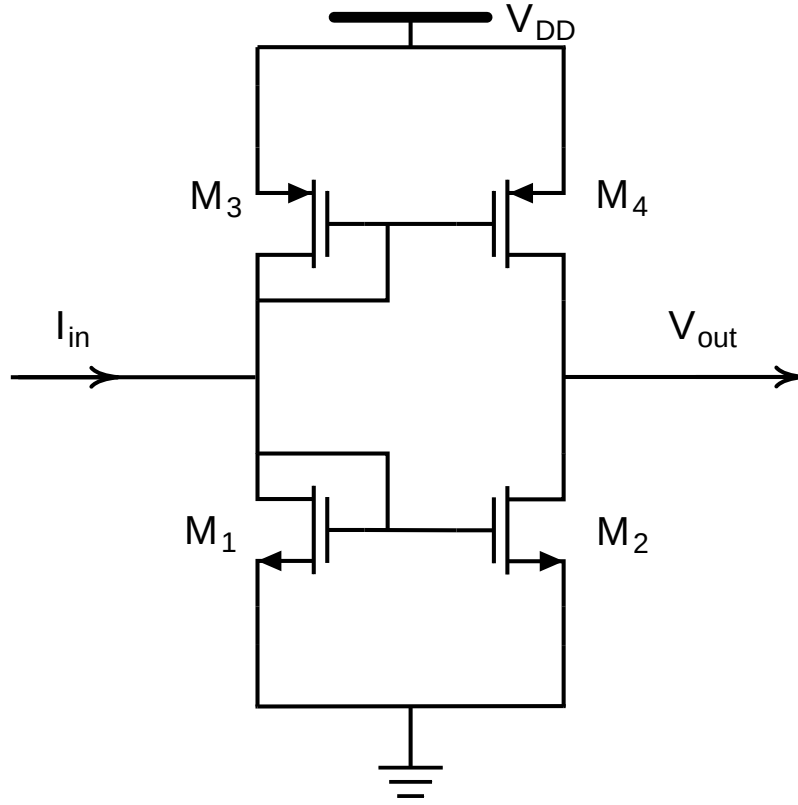
Figure 2.5: Transistor-level schematic of the current-mirror current comparator.
