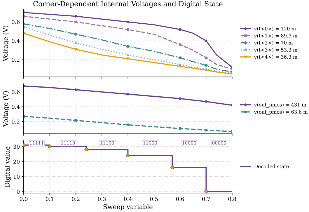
Figure 3.6: Simulated DC response of the second-architecture stage. The complementary outputs (out_nmos, out_pmos) and the internal node voltages never reach the supply rails and the transfer is visibly non-linear, the headroom shortfall predicted by equation (3.9) at the 0.8 V supply.
