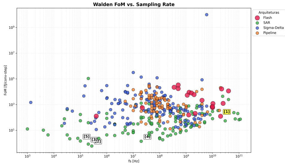
Figure 2.13: Walden FoM vs. Sampling Frequency (Flash reference [1] highlighted)
