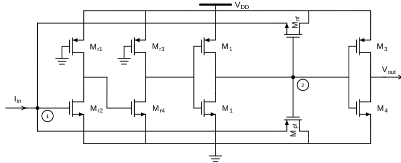
Figure 2.8: Transistor-level schematic of the hysteresis current comparator.
