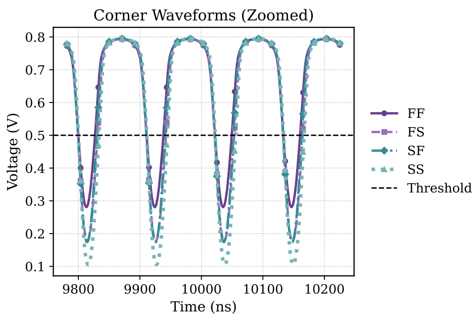
Figure 3.7: Response of the bulk-driven OTA follower across the four process corners (FF, FS, SF, SS). The output waveform diverges markedly between corners, most of all near the lower rail, the sensitivity that led to discarding the architecture.
