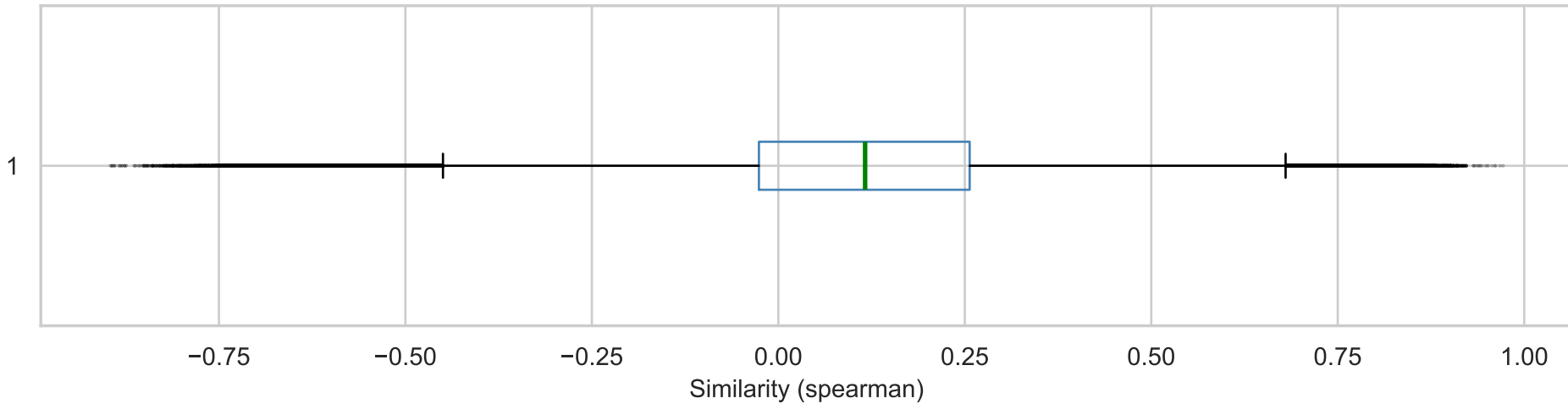
Boxplot Focal-vs-Full (spearman) | window=30 days
