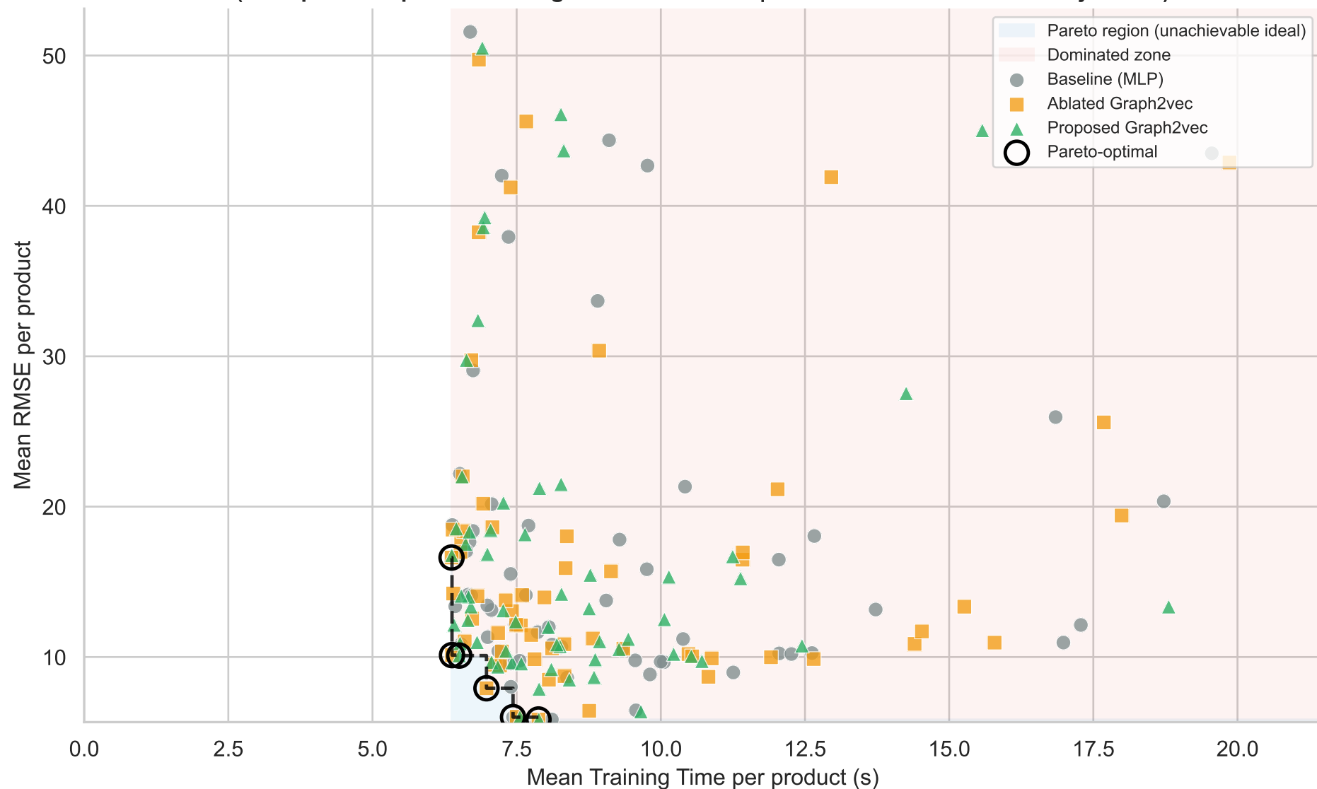
Pareto Front — Forecast Accuracy vs Training Cost (each point = 1 product averaged over 10 seeds | lower-left = ideal on both objectives)
