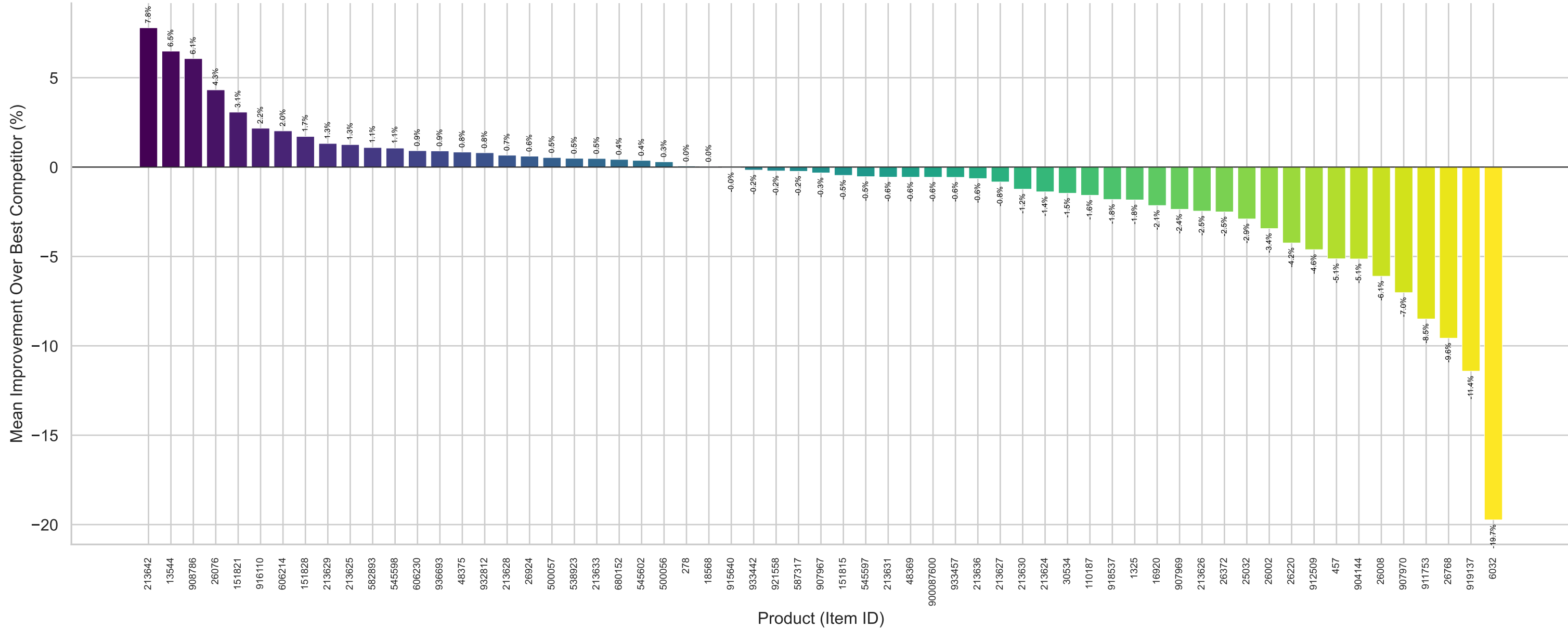
Per-Product Mean RI vs min(Baseline, Ablated) — Proposed Graph2vec Average of RMSE RI and MAE RI | Positive = Proposed beats the stronger competitor
