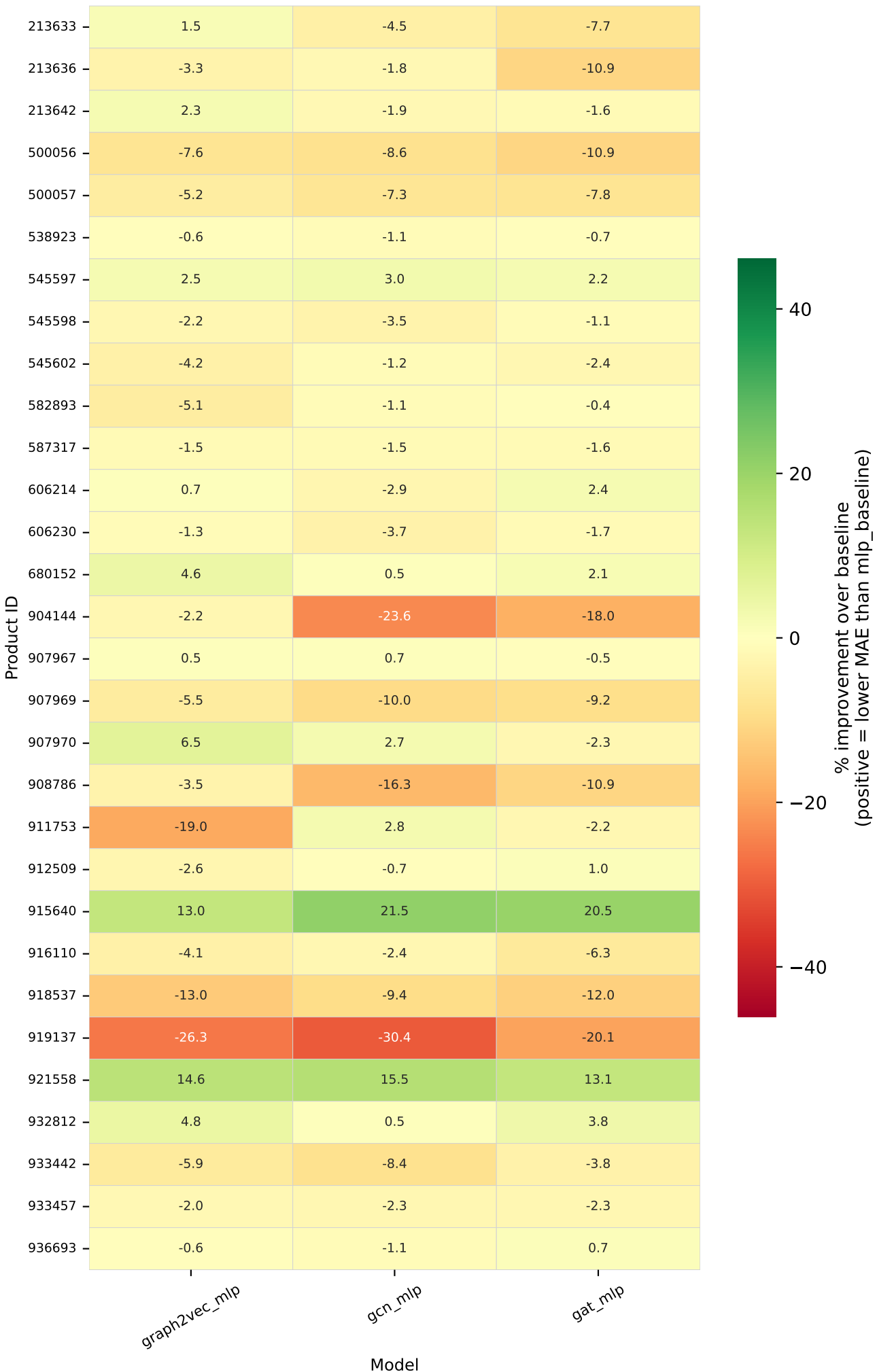
MLP — MAE % Relative Improvement over Baseline (positive = lower error) (Part 2/2)
