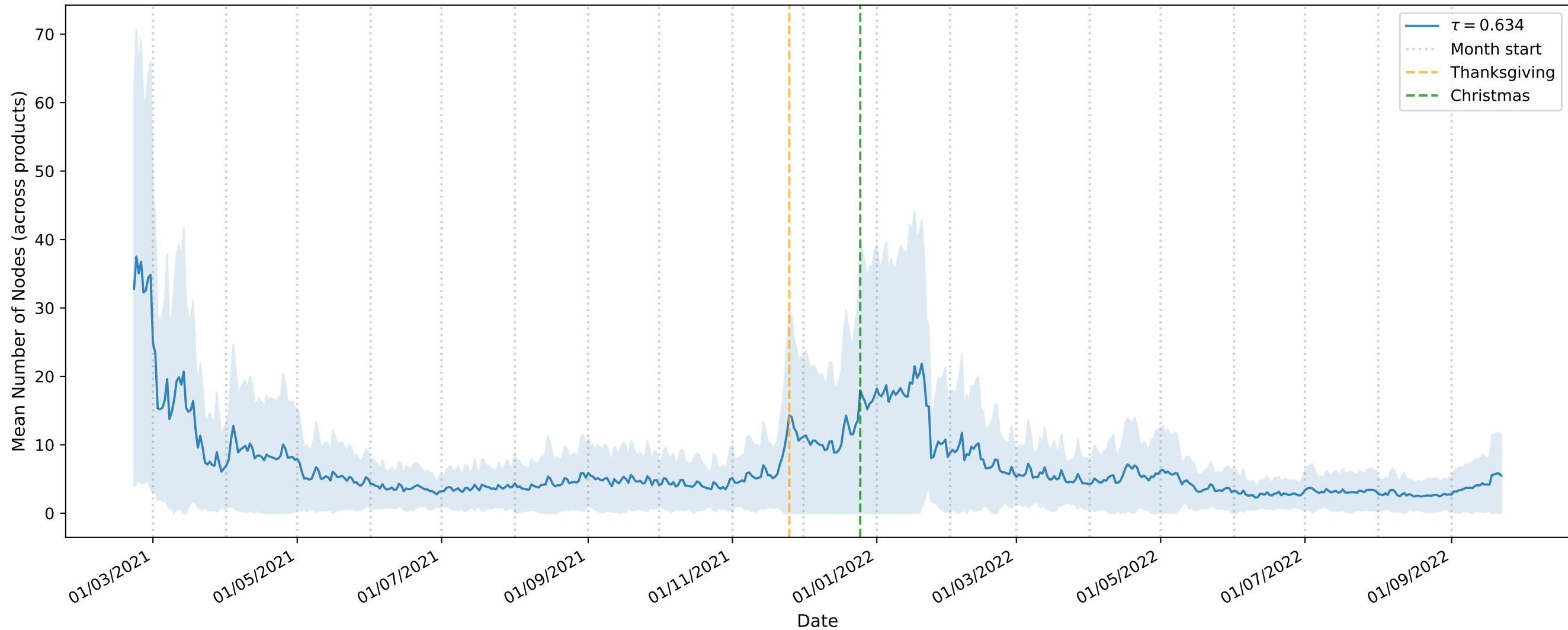
Mean Nodes per Window — spearman | window=30, step=1 | thresholds: [0.634]
