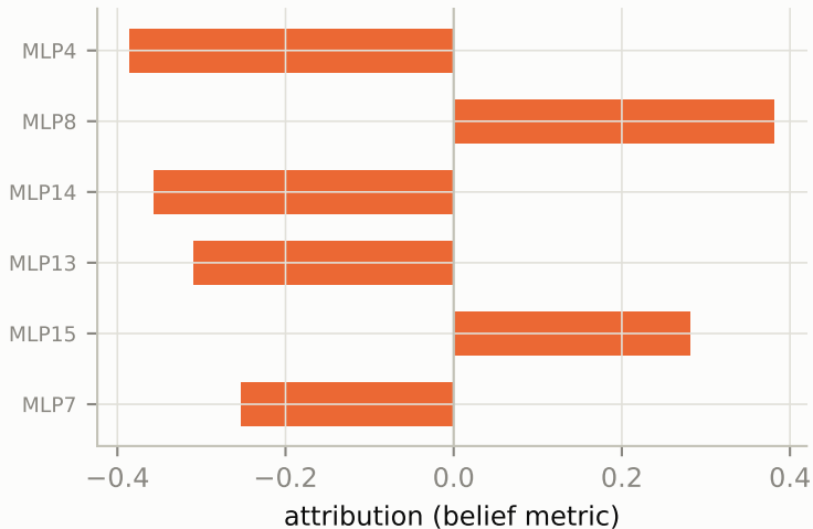
E1: attribution screening
