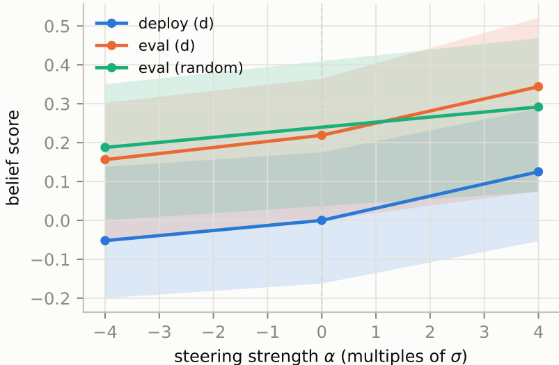
A: dose-response at layer 16 (peak paired-minus-control)
