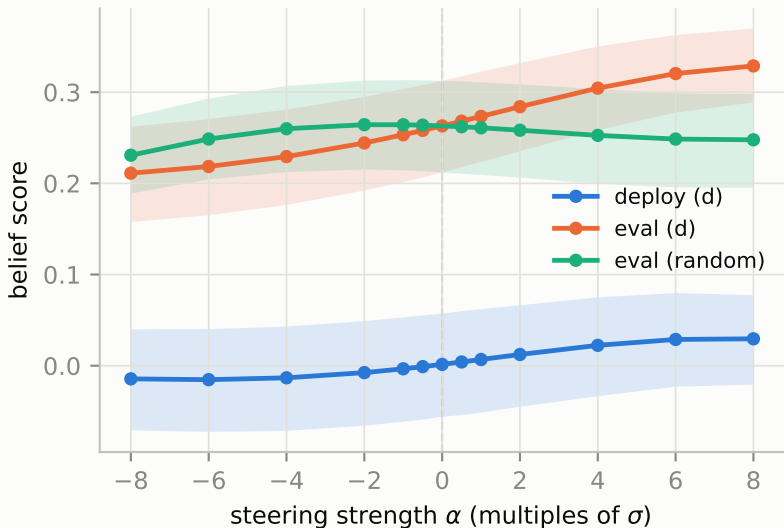
A: dose-response at layer 1 (peak paired-minus-control)
