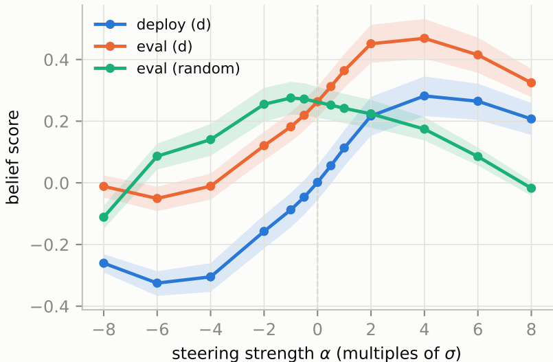
A: dose-response at layer 14 (steering sweep peak)
