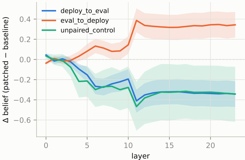
A: patching the residual stream moves the belief
