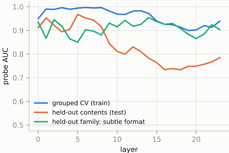
Where is eval/deploy context decodable?
