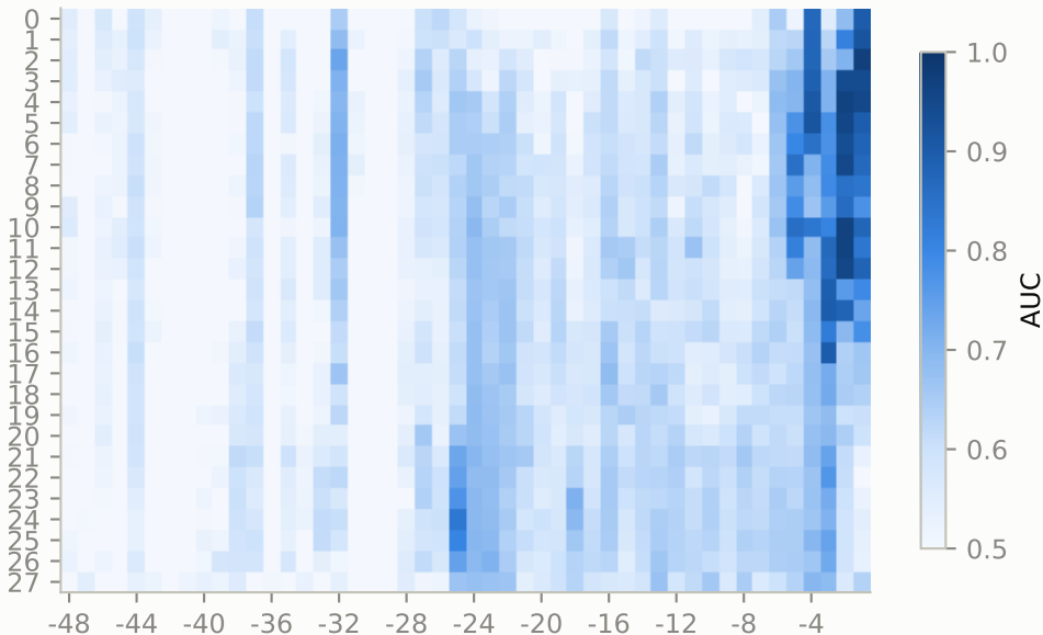
Decodability by (layer x token position)
