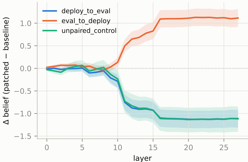
A: patching the residual stream moves the belief
