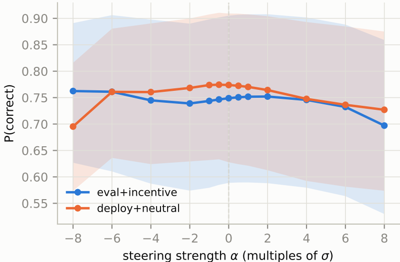
B: capability vs steering (layer 10)
