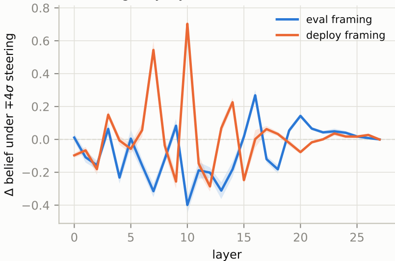
A: steering d by layer
