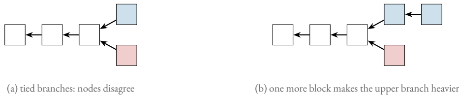
Figure 1. Branch selection. Arrows point from child to parent. In panel (a) two blocks extend the same parent and the branches carry equal work; each node keeps the one it saw first. In panel (b) a new block lands on the upper branch, which now has strictly more cumulative work; during propagation, every node that knows this state selects the upper branch, unless the lower branch has meanwhile been extended. At constant difficulty “more work” and “longer” coincide, which is how the paper, and this volume’s figures, may draw block counts.
