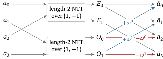
Figure 2: The length-4 transform of theorem 9.36 as a circuit. The inputs split by parity into two length-2 subtransforms, whose outputs E_0, E_1 and O_0, O_1 feed the two butterflies of theorem 9.33: each E_j is carried to outputs \hat{a}_j and \hat{a}_{j+2} with weight 1, each O_j with weights +\omega^j and -\omega^j (eq. (7)–eq. (8)); the crossing pair of weighted edges is the \times that names the butterfly.
