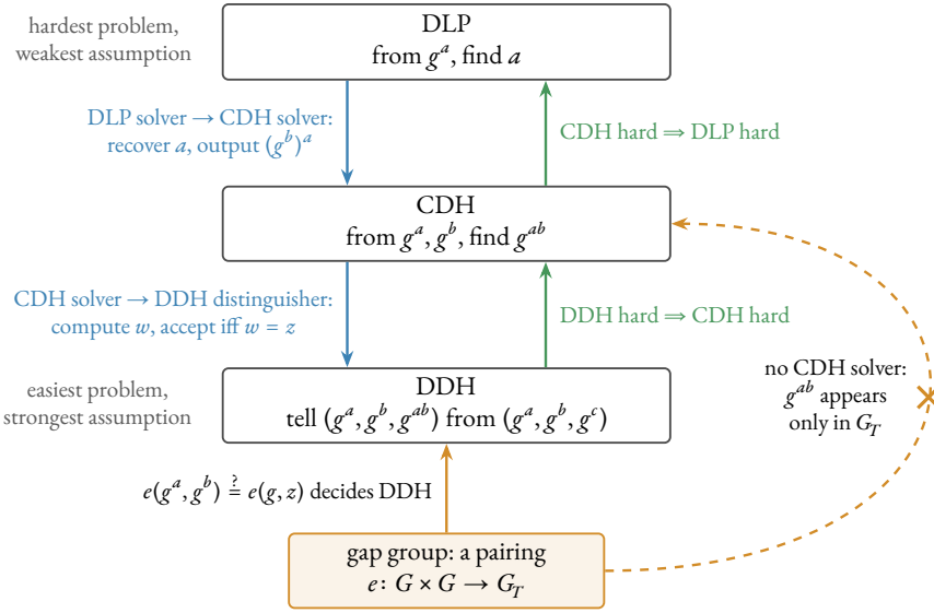
Figure 3. The three problems of §2.2 ordered by reduction. Each downward arrow (blue) converts a solver for the upper problem into one for the lower (Theorems 2.7 and 2.8), so that \text{DDH} \leq \text{CDH} \leq \text{DLP} . Each upward arrow (green) reads the same reduction as an implication between assumptions, the DDH assumption being the strongest and the DLP assumption the weakest. In a gap group (amber; Example 2.9) the pairing e decides DDH but yields g^{ab} only in the target group G_T , so it gives no CDH solver (struck edge): there DDH detaches from CDH.
