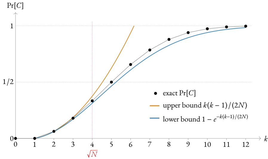
Figure 7. The collision probability \Pr[C] of Proposition 11.18 for N = 16 , against the sample count k : the exact value at each k , with the upper and lower bounds of the proposition. The upper bound exceeds 1, and so says nothing, from k = 7 on. At k = 5 , the first count beyond the threshold \sqrt{N} = 4 , the exact probability passes one half (Example 11.19).
