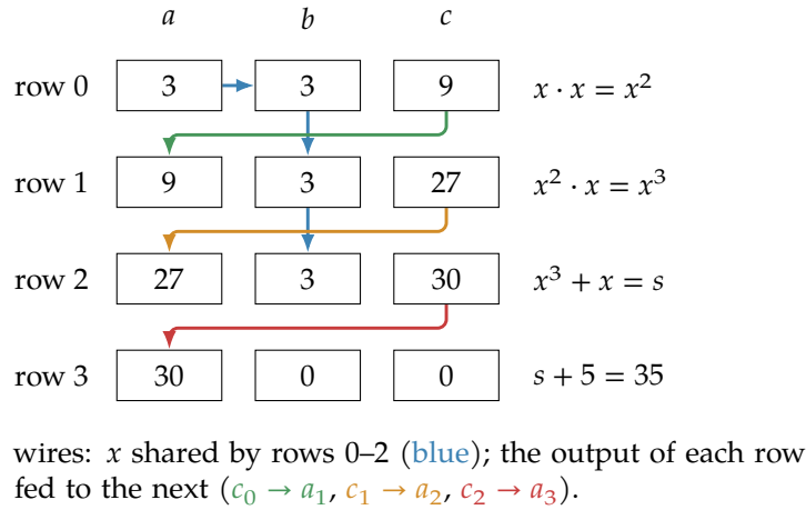
Figure 2: The four-row trace of Table 1 with the copy constraints drawn as wires. Each wire colour is one class of cells that must hold a single value: the blue wire ties the four occurrences of x , and the three coloured wires carry each row’s output c_j into the next row’s input a_{j+1} . The gates check rows; the wires make the rows one computation.
