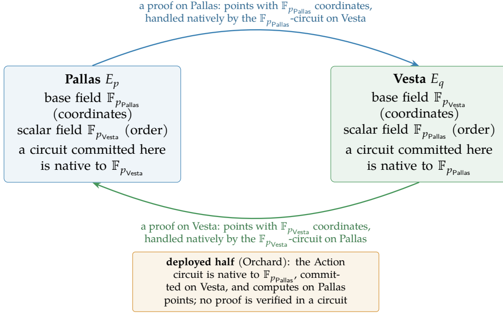
Figure 20: The Pasta 2-cycle. The base field of each curve (its coordinate field) is the scalar field of the other, so a circuit committed on Vesta (green) is native to \mathbb{F}_{p_{\text{Pallas}}} and handles Pallas points (blue) natively, and symmetrically. In a recursive chain the proofs alternate along the two arrows. Orchard (amber) uses one direction of the cycle only: Pallas arithmetic inside a Vesta-committed circuit, with no verifier circuit at all.
