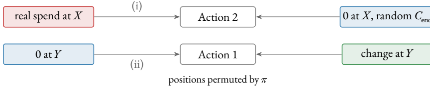
Figure 4. Assembly of Orchard-protocol bundles with n = 2 Actions
