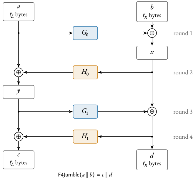
Figure 2. The four rounds of F4Jumble (Construction 3.8) on the unequal halves a ( \ell_L bytes) and b ( \ell_R bytes). Each round replaces one half by its XOR with a function of the other half, which it leaves unchanged: G_0 of a into b gives x , H_0 of x into a gives y , G_1 of y into x gives d , and H_1 of d into y gives c . Blue boxes are the extendable-output functions G_i , with \ell_R output bytes; amber boxes are the hashes H_i , with \ell_L output bytes. The names are those of the cells of Example 3.11. The structure is the content of Proposition 3.9.
