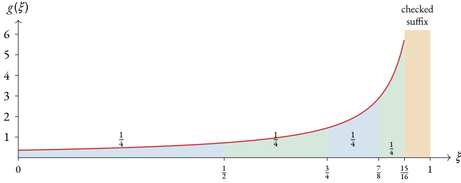
Figure 3. The FlyClient sampling density g of Construction 5.18 for c = 1/2 and k = 4 , so \delta = 1/16 and g(\xi) = 1/((1-\xi) \log 16) on [0, 15/16] . The amber strip is the suffix [15/16, 1] , checked in full, on which g vanishes. The four shaded segments [1 - c^i, 1 - c^{i+1}] , i = 0, \dots, 3 , are the invalid sets of an adversary forking at 1 - c^i with its valid weight last; each has mass 1/4 under g , and together they tile the support, which is the proof of Theorem 5.21(1).
