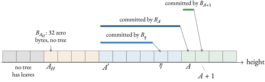
Figure 4. Committed ranges on a height axis, one cell per block, with the Heartwood activation height A_H and two later activation heights A' < A , consecutive, and A' < \eta < A . Grey: heights below A_H , a leaf of no epoch tree (Corollary 6.25). The Heartwood activation block carries the sentinel of Definition 6.12 and commits no tree. Each bar is the leaf range of the tree to which the header at the arrow's head commits: B_\eta commits B_{A'}, \dots, B_{\eta-1} ; the activation block B_A commits the whole upgrade epoch B_{A'}, \dots, B_{A-1} (Theorem 6.24(1)); and B_{A+1} commits the single leaf B_A (Theorem 6.24(2)). No bar reaches below A_H .
