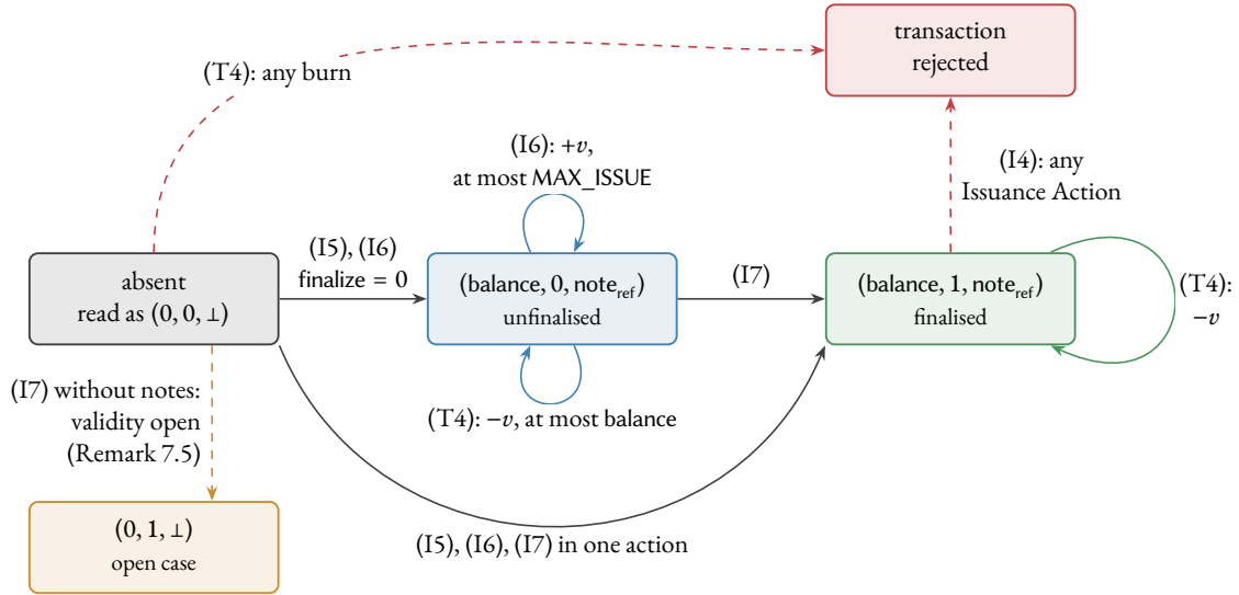
Figure 2. Transitions of one entry of the global issuance state of Definition 7.1. Solid edges are accepted transitions, labelled with the rules of Construction 7.3 that take them. The first issuance, by (I5) and (I6), creates the entry together with its reference note, as in Lemma 7.6; one action may also issue and finalise at once. The unfinalised entry grows under (I6), up to \text{MAX\_ISSUE} , and shrinks under (T4), down to 0; the finalised entry only shrinks under (T4), again down to 0, and every Issuance Action on it is rejected by (I4), as in Proposition 7.8. A burn of an absent entry is rejected by (T4). The dashed edge to (0, 1, \perp) is case (b) of Remark 7.5, an open problem.
