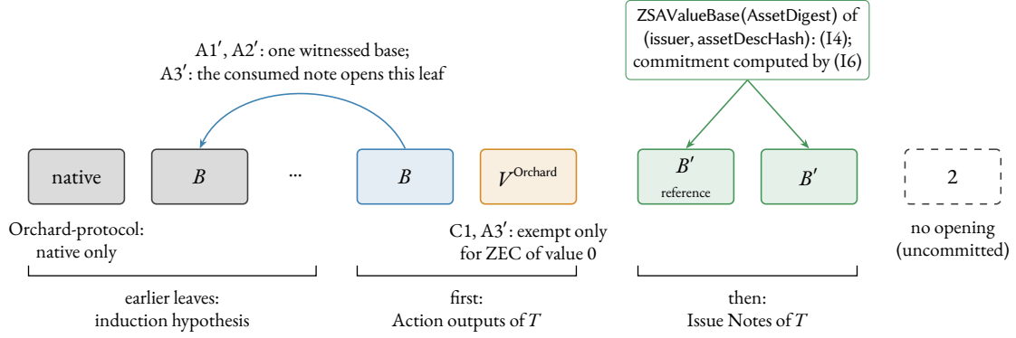
Figure 3. Provenance of Asset Bases in the tree, the induction of Lemma 9.3.
