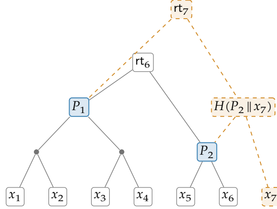
Figure 1: The range M_6 over x_1, \dots, x_6 in single-rooted form (solid): the root rt_6 has left child P_1 , the perfect range over x_1, \dots, x_4 , and right child P_2 = H(x_5 \parallel x_6) , the perfect range over x_5, x_6 . The nodes P_1 and P_2 are the peaks of Definition 3.4; P_2 is the first perfect node on the right spine of M_6 , whose last node is the leaf x_6 . Dashed: appending x_7 creates only the nodes H(P_2 \parallel x_7) and rt_7 = H(P_1 \parallel H(P_2 \parallel x_7)) ; the nodes P_1, P_2 and every node beneath them are shared by M_6 and M_7 .
