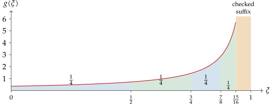
Figure 3: The FlyClient sampling density g of Construction 5.18 for c = 1/2 and k = 4 , so \delta = 1/16 and g(\xi) = 1/((1 - \xi) \log 16) on [0, 15/16] . The amber strip is the suffix [15/16, 1] , checked in full, on which g vanishes. The four shaded segments [1 - c^i, 1 - c^{i+1}] , i = 0, \dots, 3 , are the invalid sets of an adversary forking at 1 - c^i with its valid weight last; each has mass 1/4 under g , and together they tile the support, which is the proof of Theorem 5.21(1).
