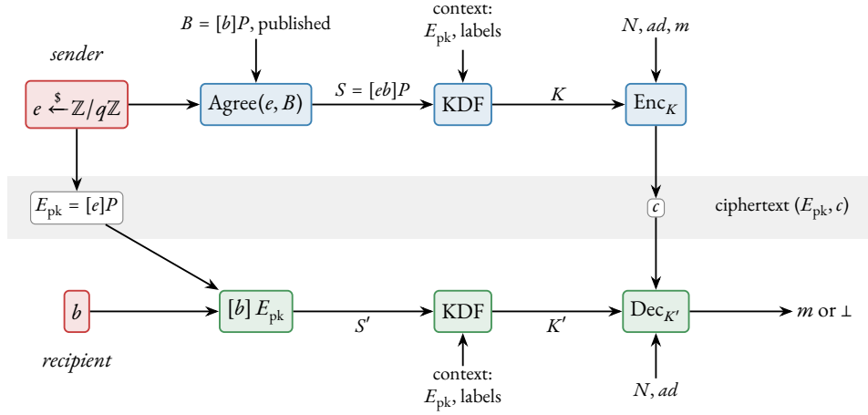
Figure 11. Hybrid public-key encryption, Construction 7.22. The sender (blue lane) samples the ephemeral e , publishes E_{pk} = [e]P , agrees S = [eb]P with the recipient's static key B , derives K from S and a context containing E_{pk} , and encrypts m under K with nonce N and associated data ad . The ciphertext (E_{pk}, c) (grey band) is all that crosses the channel. The recipient (green lane) mirrors the sender with its secret b : S' = [b]E_{pk} , then K' , then decryption, which returns m on an honest ciphertext and, except with negligible probability, \perp on a tampered one. Red marks the two secret scalars.
