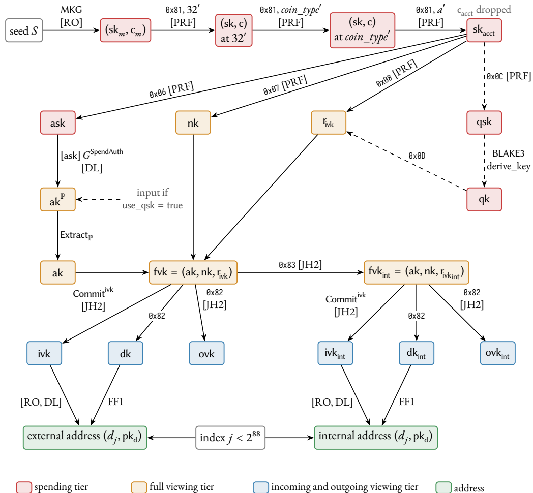
Figure 1. Derivation of the keys of one account, from the seed S through the master key and the hardened levels 32' , \text{coin\_type}' and a' to the account spending key \text{sk}_{\text{acct}} , whose chain code is dropped; then the key components, the full viewing key \text{fvk} , the internal full viewing key \text{fvk}_{\text{int}} , the incoming and outgoing viewing keys of each scope, and the addresses at each index j . Solid edges are those of a key with \text{use\_qsk} = \text{false} ; dashed edges are the \text{use\_qsk} = \text{true} sources of \text{ak}^{\text{P}} , an input, and of \text{r}_{\text{ivk}} , through \text{qsk} and \text{qk} . Each derivation edge carries its expansion byte or operation; unlabelled edges are projections into a tuple or inputs. Each one-way edge also carries the assumption under which it is one-way: PRF, the Ironwood Guide ’s Assumption “Pseudorandomness of PRF expansion” (§“Pseudorandom functions and field reductions”); RO, a random oracle (BLAKE2b under ZcashIP320rchard for MKG, GroupHash for the diversified base); DL, its Assumption “Discrete logarithms on Pallas”; JH2, the joint hiding assumption of both scopes stated in §2.5. Colours give the lowest key tier that computes a node. The separations the figure depicts are proved in §2.5.
