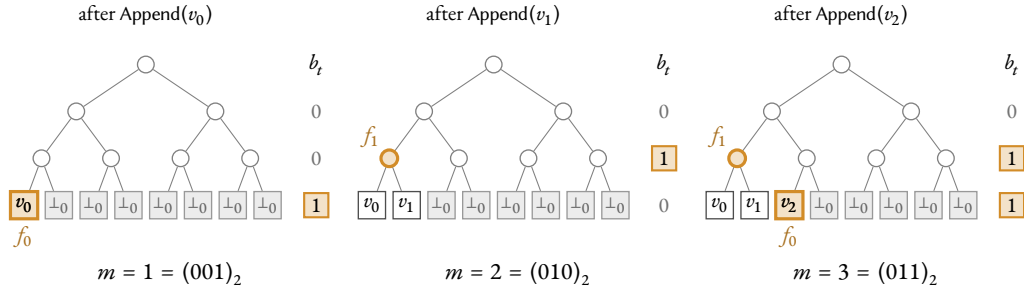
Figure 17. The frontier of Definition 10.19 across the three appends of Example 10.21, on a tree of depth d = 3 ; grey leaves hold the empty-leaf value \perp_0 . The frontier labels (amber) sit at the levels t of the set bits b_t of the leaf count m , shown beside each tree: after v_0 it is f_0 = v_0 ; appending v_1 carries f_0 into f_1 = \text{NodeHash}_1(v_0, v_1) , as (001)_2 + 1 carries into (010)_2 ; appending v_2 deposits f_0 = v_2 and leaves f_1 in place.
