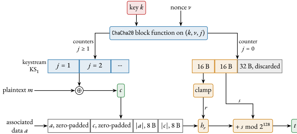
Figure 9. The scheme ChaCha20-Poly1305 of Construction 6.18. The ChaCha20 block function (blue) on the key k (red) and nonce v yields one 64-byte block per counter j . Block 0 (amber) is the one-time Poly1305 key: its first 16 bytes, clamped, form r , the next 16 form s , and the last 32 are discarded. The blocks from counter 1 on form the keystream KS_1 , XORed into m to give c . The Poly1305 MAC (amber) hashes, under r , the zero-padded a and c followed by their 8-byte little-endian lengths, and adds the pad s modulo 2^{128} to give the tag t ; the ciphertext is (c, t) (green). Reserving counter 0 for the MAC key is domain separation: the MAC key and the keystream are outputs of the cipher at distinct counters (Remark 6.21).
