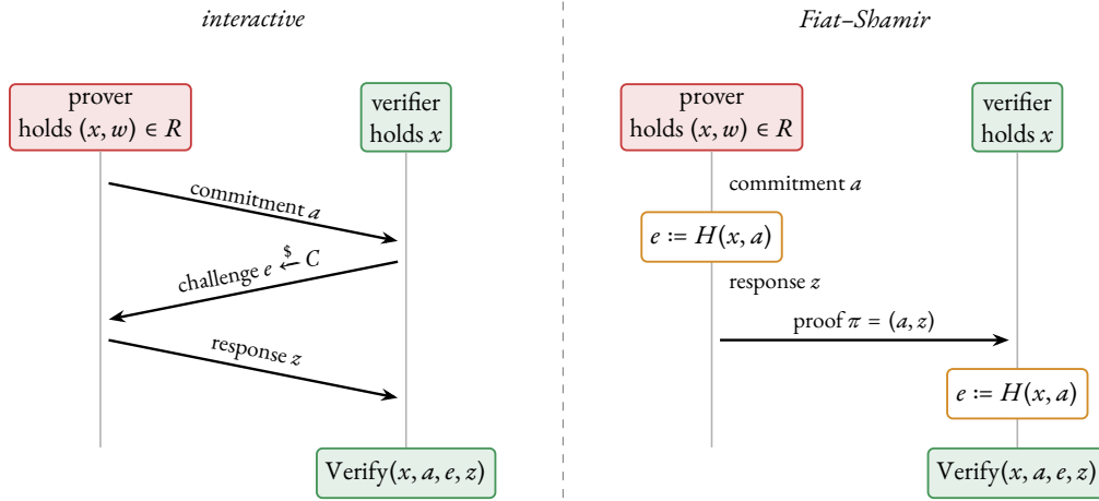
Figure 15. A Sigma-protocol (left), Definition 9.12, and its Fiat-Shamir transform (right), Definition 9.19. Left: the prover, holding w with (x, w) \in R , sends the commitment a ; the verifier answers with a uniform challenge e \in C ; the prover sends the response z , and the verifier decides by \text{Verify}(x, a, e, z) . The three messages trace the zigzag of a capital \Sigma . Right: the hash H (amber) replaces the verifier's challenge. The prover computes e := H(x, a) itself and sends the single proof string \pi = (a, z) ; the verifier recomputes e from x and a and applies the same predicate. Only the prover holds a secret (red).
