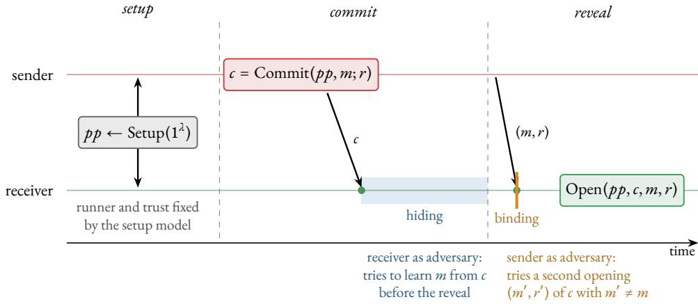
Figure 7. The three phases of Remark 4.2. In the setup phase, Setup produces the public parameters pp for both parties; who runs it, and whether that party is trusted, is fixed by the setup model (Remark 4.3). In the commit phase the sender (red), holding the secret (m, r) , transmits c = \text{Commit}(pp, m; r) and nothing else; from that point until the reveal, hiding (blue) protects the sender against a receiver who tries to learn m from c . In the reveal phase the sender transmits the opening (m, r) and the receiver (green) runs Open; at that point binding (amber) protects the receiver against a sender who could open c to a second message.
