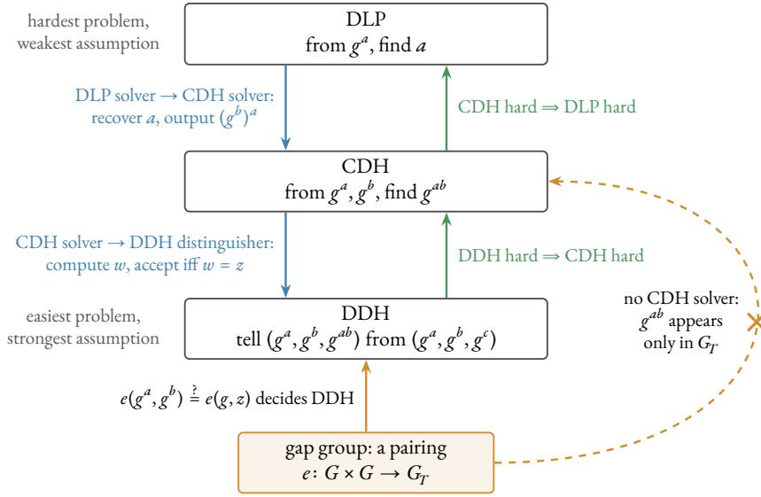
Figure 3. The three problems of §2.2 ordered by reduction. Each downward arrow (blue) converts a solver for the upper problem into one for the lower (Theorems 2.7 and 2.8), so that \text{DDH} \leq \text{CDH} \leq \text{DLP} . Each upward arrow (green) reads the same reduction as an implication between assumptions, the DDH assumption being the strongest and the DLP assumption the weakest. In a gap group (amber; Example 2.9) the pairing e decides DDH but yields g^{ab} only in the target group G_T , so it gives no CDH solver (struck edge): there DDH detaches from CDH.
