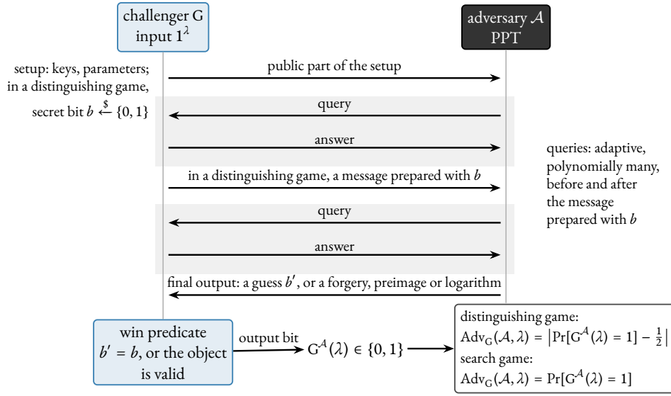
Figure 1. The security game of Definition 1.15, with no scheme instantiated. The challenger (blue) runs the setup on 1^\lambda , sampling the secret bit b in a distinguishing game, and passes the public part of the setup to the adversary (black). It answers the adversary’s queries (grey bands), before and after it sends, in a distinguishing game, a message prepared with b , and it receives the final output: a guess b' in a distinguishing game; a forgery, preimage or discrete logarithm in a search game. The win predicate turns the run into the output bit G^{\mathcal{A}}(\lambda) , and the advantage is read off its distribution. The pseudorandomness game of Example 1.17, the PRF game of Definition 5.4, the CPA game of Definition 6.4 and the unforgeability game of Definition 8.2 are instances.
