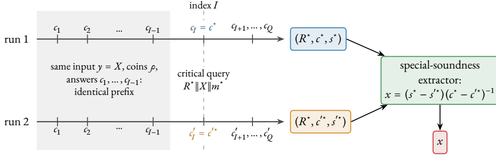
Figure 13. The fork in the proof of Theorem 8.18, an execution of the forking algorithm F_B of Theorem 8.17. Both runs of B take the same input y = X and coins \rho , and answer the first I - 1 distinct hash queries with the same c_1, \dots, c_{I-1} (grey band), so they coincide up to the I -th query, the critical input R^* \| X \| m^* . There run 1 receives c_I = c^* (blue) and run 2 a fresh c'_I = c'^* (amber), and each continues with its own remaining challenges. When both forge with the same index I and c^* \neq c'^* , the outputs are two accepting transcripts with the common commitment R^* and distinct challenges, from which the extractor of Theorem 8.8 computes the discrete logarithm x of X (red).
