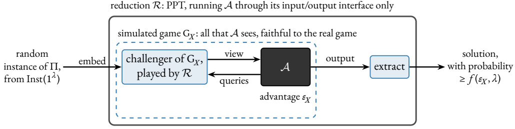
Figure 2. A black-box reduction, Definition 1.20, in the four-step structure of §1.5. The reduction \mathcal{R} (outer frame) receives a random instance of \Pi and embeds it in a simulated security game G_X (blue, dashed), whose challenger it plays. The adversary \mathcal{A} (black) is opaque: the reduction reaches it only through its input/output interface. The dashed boundary is all that \mathcal{A} sees; the simulation makes it faithful to the real game, so that the advantage \varepsilon_X of \mathcal{A} carries over. From the output of \mathcal{A} , the reduction extracts a solution to the instance, with success probability at least f(\varepsilon_X, \lambda) .
