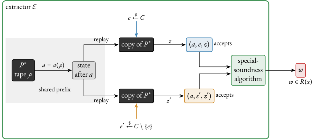
Figure 14. The extractor in the proof of Theorem 9.13, on a run that ends in a collision. The extractor \mathcal{E} (frame) holds the prover P^* (black) as a subroutine. Fixing the random tape \rho fixes the commitment a = a(\rho) , and \mathcal{E} replays P^* from the state just after a was emitted (grey band), once with the challenge e and once with a fresh e' \neq e . If both transcripts (a, e, z) and (a, e', z') accept, they form a collision, from which the special-soundness algorithm of Definition 9.12 computes a witness w \in R(x) (red). The rewinding is legitimate because P^* is code that \mathcal{E} runs, not a live counterpart (Remark 9.8). The fresh probes by which the proof bounds the expected running time are not drawn.
