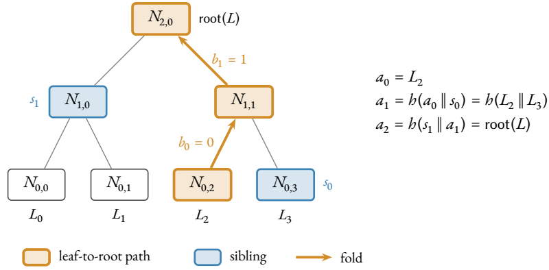
Figure 16. The authentication path of Example 10.10 in the depth-2 tree of Example 10.3. The path from the leaf at index i = 2 = (10)_2 to the root, N_{0,2}, N_{1,1}, N_{2,0} , is amber; the siblings s_0 = N_{0,3} and s_1 = N_{1,0} , which form \pi_2 with the bits, are blue. The bit b_0 = 0 places the running value on the left at level 0 and b_1 = 1 on the right at level 1; the fold (4) at the right recomputes the root from L_2 and the two siblings alone.
