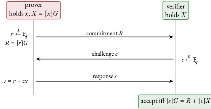
Figure 12. The three moves of Construction 8.6 in G = \langle G \rangle of prime order q . The prover, holding the witness x of the statement X = [x]G , commits to a fresh nonce r by sending R = [r]G ; the verifier answers with a uniform challenge c ; the prover responds with s = r + cx in \mathbb{F}_q . The verifier accepts iff [s]G = R + [c]X , equation (2); only the prover holds a secret (red).
