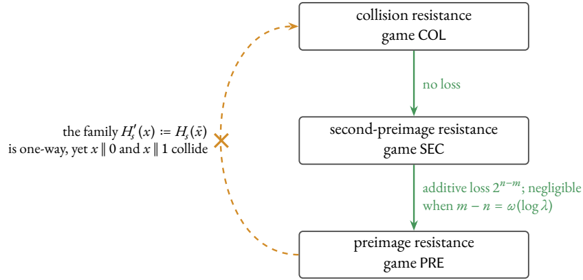
Figure 4. The implications of Proposition 3.8 for a compressing keyed family H with challenge length m > n . Each solid arrow (green) is an implication, proved by a reduction that turns an adversary against the lower notion into one against the upper: collision resistance yields second-preimage resistance with no loss, and second-preimage resistance yields preimage resistance up to the additive loss 2^{n-m} , negligible when m - n = \omega(\log \lambda) . The struck edge (amber) is Example 3.9: the family H' , which deletes the last bit of its input before hashing, is one-way whenever H is, yet x \parallel 0 and x \parallel 1 collide for every x , so preimage resistance does not imply collision resistance.
