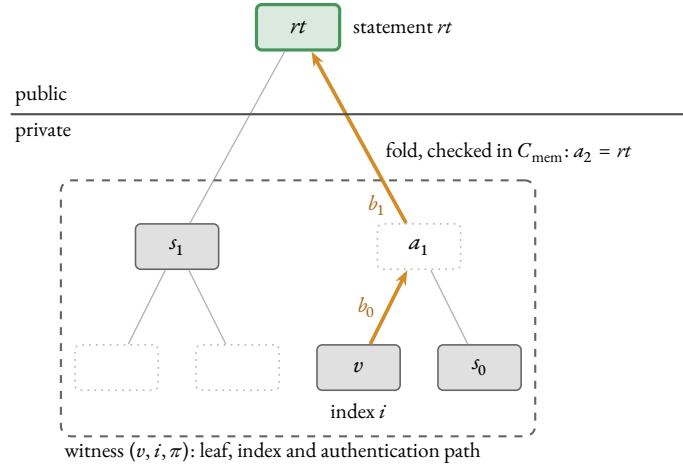
Figure 18. The relation R_{\text{mem}} of Definition 10.27 on the depth-2 tree, for the path of Example 10.10 ( i = 2 ). Above the divider, the root rt alone is the public statement (green). Below it, the witness (grey, boxed) is the leaf v , its index i , entering the circuit only through the bits b_0 and b_1 , and the siblings s_0 and s_1 . The circuit C_{\text{mem}} of Construction 10.28 performs the fold (4) (amber) through the intermediate value a_1 and enforces a_2 = rt ; dotted nodes are neither public nor part of the witness.
