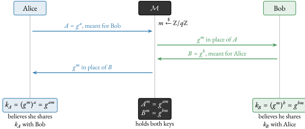
Figure 10. The attack of Definition 7.13. The adversary \mathcal{M} (black) intercepts the messages of Alice and Bob and substitutes g^m in each direction, so that two independent Diffie–Hellman sessions run: one between Alice and \mathcal{M} (blue), with key k_A = g^{am} , and one between \mathcal{M} and Bob (green), with key k_B = g^{bm} . The adversary computes both keys from its own m and the received A and B ; each victim’s view is an honest run of the protocol.
