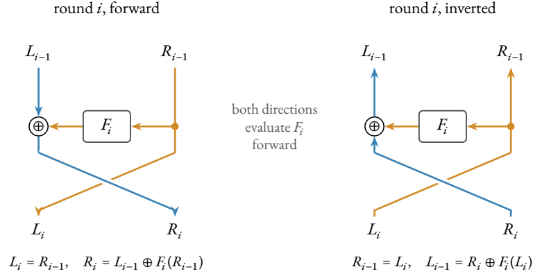
Figure 8. One round of the balanced Feistel network of Definition 5.16 (left) and its inversion (right). Forward, R_{i-1} (amber) passes unchanged to L_i and also enters F_i , whose output is XORed into L_{i-1} (blue) to give R_i ; the rails then cross. The right panel is the same wiring read from bottom to top, the decryption direction: L_i returns to the right rail as R_{i-1} and enters F_i , and XORing its output into R_i recovers L_{i-1} (Proposition 5.17). In both directions F_i is evaluated forward, so it need not be invertible.
