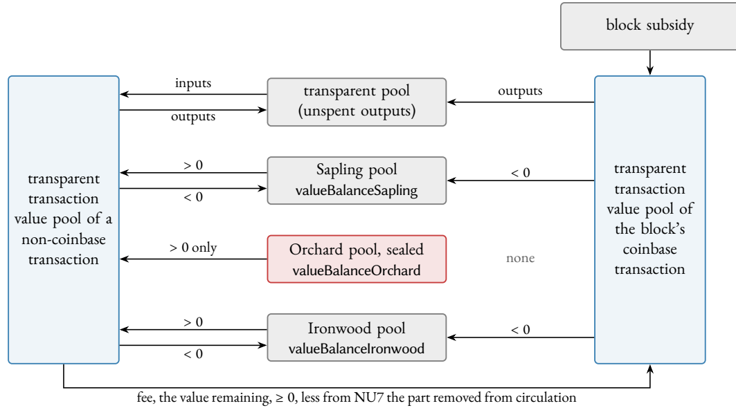
Figure 6. The flows of value that the rules permit between the pools of the Orchard protocol, the Sapling pool and the transparent pool, the chain value pool of the unspent transparent outputs. Every flow passes through the transparent transaction value pool of a transaction, drawn as a hub for a non-coinbase transaction (left) and for the block’s coinbase transaction (right). An arrow between a hub and a shielded pool is labelled by the sign of that pool’s balancing value, positive out of the pool and negative into it; every such arrow crosses the turnstile, its amount public. No arrow enters the sealed Orchard pool (rule (ii)), and the coinbase transaction has no Orchard-pool Action (rule (iii)); it consumes no Ironwood-pool note of non-zero value (rule (iv)) and no Sapling note, and its hub receives the block subsidy and the fees of the block’s other transactions, less from NU7 the part of those fees removed from circulation, which no pool receives (“The balancing value”, §8.2). The Sprout pool, which no transaction of version 5 or 6 reaches (§11.2), and the deferred development fund pool of ZIP 209 are not drawn.
