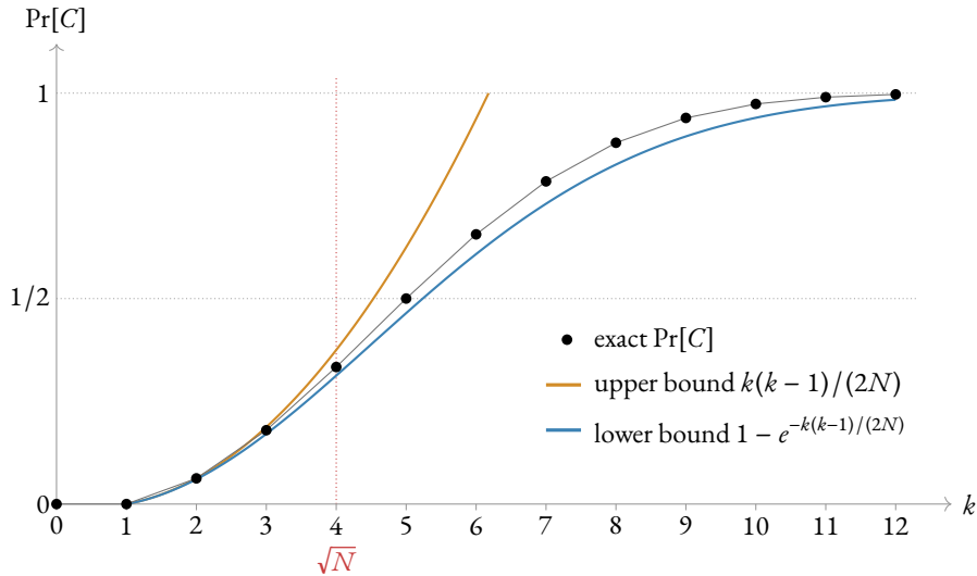
Figure 7. The collision probability \Pr[C] of Proposition 11.18 for N = 16 , against the sample count k : the exact value at each k , with the upper and lower bounds of the proposition. The upper bound exceeds 1, and so says nothing, from k = 7 on. At k = 5 , the first count beyond the threshold \sqrt{N} = 4 , the exact probability passes one half (Example 11.19).
