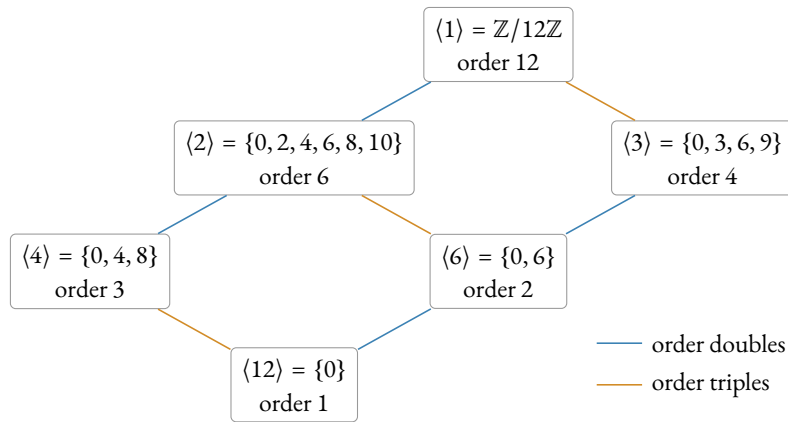
Figure 1. The subgroup lattice of \mathbb{Z}/12\mathbb{Z} . By Theorem 3.24(3) there is one subgroup \langle 12/d \rangle for each divisor d of 12, of order d . An edge joins two subgroups when the lower is contained in the upper with no subgroup between them, which happens exactly when the quotient of their orders is prime: blue edges double the order, orange edges triple it. Inclusion of subgroups matches divisibility of their orders, so the diagram is also the divisor lattice of 12.
