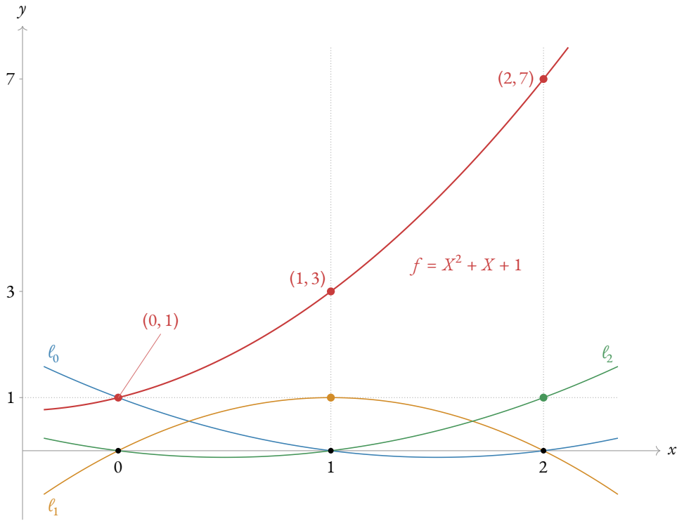
Figure 2. The Lagrange basis polynomials \ell_0, \ell_1, \ell_2 for the nodes 0, 1, 2 of Example 5.31, read as functions on \mathbb{R} . Each takes the value 1 at its own node and vanishes at the other two, the delta property (4). The interpolant f = 1 \cdot \ell_0 + 3 \cdot \ell_1 + 7 \cdot \ell_2 = X^2 + X + 1 passes through (0, 1), (1, 3) and (2, 7); at the node 0 it meets \ell_0 , since y_0 = 1 .
