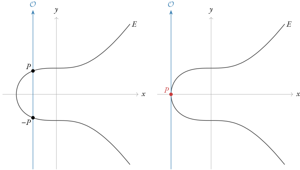
Figure 6. The vertical cases of the group law on the real points of E : y^2 = x^3 + 5 . Left: the line x = -1 through P = (-1, 2) and -P = (-1, -2) meets E a third time only at the point at infinity \mathcal{O} , so P + (-P) = \mathcal{O} . Right: at P = (-\sqrt[3]{5}, 0) , the only real point with y = 0 , the tangent x = -\sqrt[3]{5} is vertical, so [2]P = \mathcal{O} . Each arrow points in the vertical direction, where both lines pass through \mathcal{O} (§10.2).
