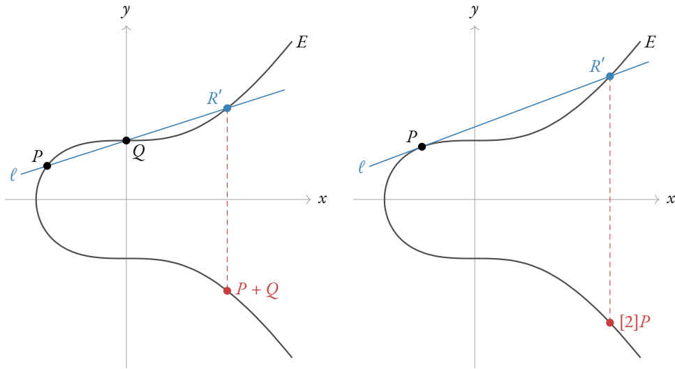
Figure 5. The chord-and-tangent law of Definition 10.7 on the real points of E : y^2 = x^3 + 5 . Left: the chord \ell through P and Q meets E a third time at R' , and P + Q is the reflection of R' across the x -axis. Right: the tangent \ell at P = (-1, 2) , of slope 3/4 , meets E again at R' = (41/16, 299/64) , so [2]P = (41/16, -299/64) , as (13) computes.
