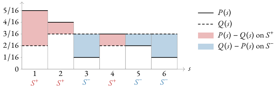
Figure 8. Statistical distance as area, for the distributions P = (5, 4, 1, 3, 2, 1)/16 and Q = (2, 3, 3, 2, 3, 3)/16 on S = \{1, \dots, 6\} , drawn as overlaid bar charts of unit width. The shading between the two bar heights has total area \sum_s |P(s) - Q(s)| = 10/16 . Its part over S^+ = \{1, 2, 4\} , where P exceeds Q , and its part over S^- = \{3, 5, 6\} each have area 5/16 , and \Delta(P, Q) = 5/16 is half the total.
