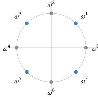
Figure 3. The eight 8-th roots of unity in \mathbb{C} , equally spaced on the unit circle at angles 2\pi k/8 , with \omega = e^{2\pi i/8} . The four primitive ones ( k = 1, 3, 5, 7 , exactly the k coprime to 8; marked in colour) each generate the whole cycle; the grey points \omega^0 = 1, \omega^2 = i, \omega^4 = -1, \omega^6 = -i have orders 1, 4, 2, 4 and generate proper subgroups. Over a finite field the cyclic group structure persists without the geometry of the circle.
