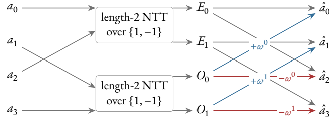
Figure 4. The length-4 transform of Example 9.39 as a circuit. The inputs split by parity into two length-2 subtransforms, whose outputs E_0, E_1 and O_0, O_1 feed the two butterflies of Remark 9.36: each E_j is carried to outputs \hat{a}_j and \hat{a}_{j+2} with weight 1, each O_j with weights +\omega^j and -\omega^j (Eq. (7)–Eq. (8)); the crossing pair of weighted edges is the \times after which the butterfly is named.
