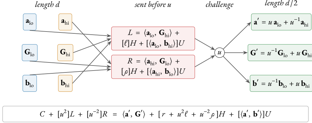
Figure 7. One fold. The three vectors of length d (left; low halves in blue, high halves in amber) determine the two cross terms L and R (red): L from \mathbf{a}_{lo} , \mathbf{G}_{hi} and \mathbf{b}_{hi} , R from the complementary halves, both sent before the challenge u is drawn. The challenge then folds all three vectors to length d/2 (green). The identity beneath is equation (14): the folded commitment has the same three-part shape as the original, over the folded vectors, with the cross terms absorbed at weights u^2 and u^{-2} .
