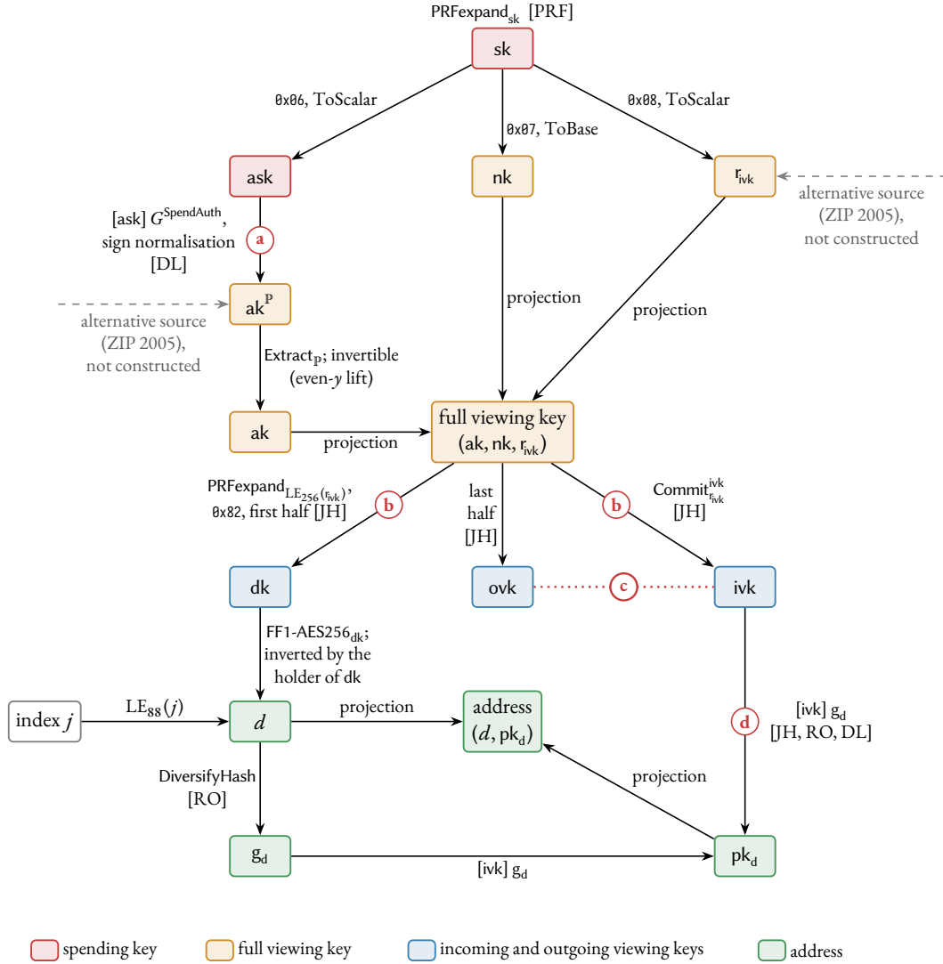
Figure 1. Derivation graph of a key generated with use\_qsk = \text{false} , from the spending key sk to the address (d, pk_d) . Each edge carries its operation, and each one-way edge also carries, in brackets, the assumption under which it is one-way: PRF, Assumption 2.12; DL, Assumption 2.22; JH, Assumption 3.13; RO, Assumption 2.8. Each one-way edge is a PRF call, a scalar multiplication, the joint hiding assumption or GroupHash as a random oracle; bundling edges invert by projection, \text{Extract}_P by the even- \gamma lift, and the FF1 edge is inverted by the holder of dk . The edges out of sk are one-way under Assumption 2.12, since an algorithm recovering sk from (ask, nk, r_{ivk}) distinguishes \text{PRFexpand}_{sk} from a random function. Colours give the lowest key tier that computes a node; the index j is uncoloured. The dashed edges into ak^P and r_{ivk} mark the alternative source of ZIP 2005, not constructed. Markers (a) to (d) are the four separations that Proposition 3.18 proves; no other separation is claimed.
