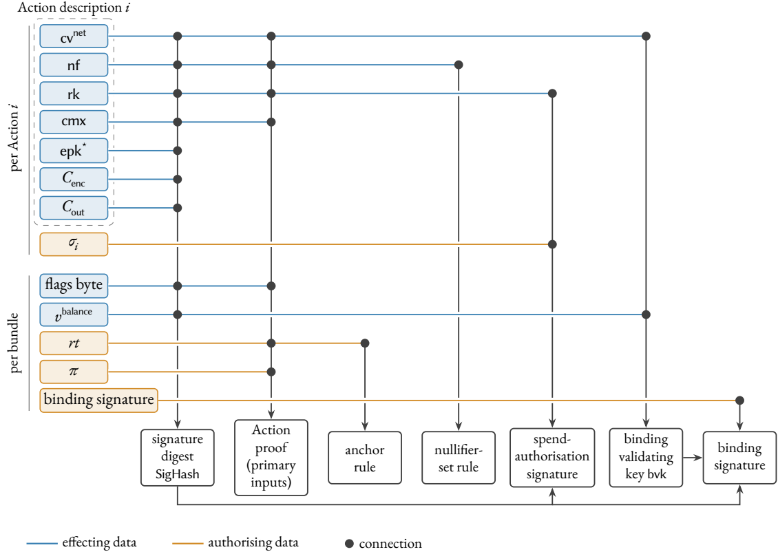
Figure 4. The public data of one bundle and the checks that consume them.
