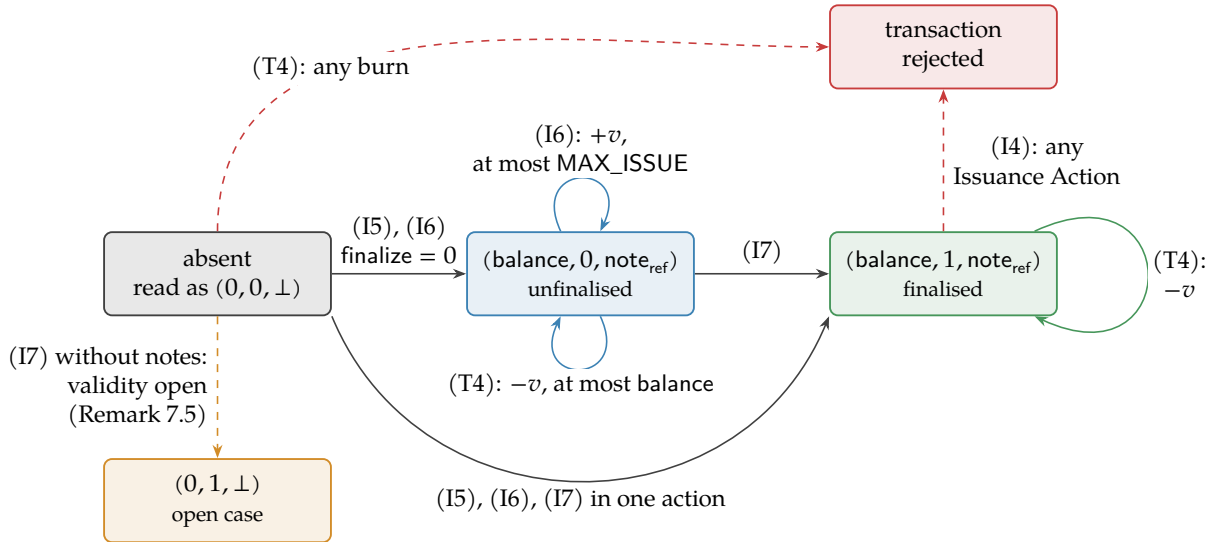
Figure 2: Transitions of one entry of the global issuance state of Definition 7.1. Solid edges are accepted transitions, labelled with the rules of Construction 7.3 that take them. The first issuance, by (I5) and (I6), creates the entry together with its reference note, as in Lemma 7.6; one action may also issue and finalise at once. The unfinalised entry grows under (I6), up to MAX_ISSUE, and shrinks under (T4), down to 0; the finalised entry only shrinks under (T4), again down to 0, and every Issuance Action on it is rejected by (I4), as in Proposition 7.8. A burn of an absent entry is rejected by (T4). The dashed edge to (0, 1, \perp) is case (b) of Remark 7.5, an open problem.
