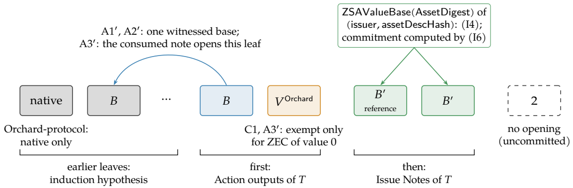
Figure 3: Provenance of Asset Bases in the tree, the induction of Lemma 9.3. One transaction T appends its leaves in the order of Definition 7.4: the outputs of its Actions, then its Issue Notes. Earlier leaves (grey) satisfy the induction hypothesis; a leaf appended by an Orchard-protocol Action opens only with V^{\text{Orchard}} . An Action output of a Custom Asset B (blue) inherits B from an earlier leaf through A1' , A2' and A3' ; C1 confines the exemption from membership to ZEC (amber). The Asset Base B' of an Issue Note (green) is derived by the validator from issuer and assetDescHash by (I4), and its commitment computed by (I6). The empty leaf 2 opens to no note.
