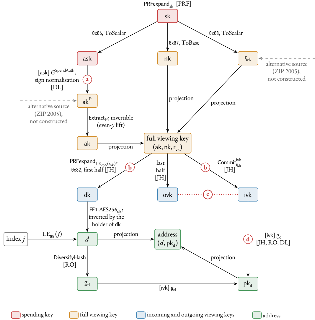
Figure 1. Derivation graph of a key generated with use_qsk = false , from the spending key sk to the address (d, pk_d) . Each edge carries its operation, and each one-way edge also carries, in brackets, the assumption under which it is one-way: PRF, Assumption 2.12; DL, Assumption 2.22; JH, Assumption 3.13; RO, Assumption 2.8. Each one-way edge is a PRF call, a scalar multiplication, the joint hiding assumption or GroupHash as a random oracle; bundling edges invert by projection, \text{Extract}_p by the even- \gamma lift, and the FF1 edge is inverted by the holder of dk . The edges out of sk are one-way under Assumption 2.12, since an algorithm recovering sk from (ask, nk, r_{ivk}) distinguishes \text{PRFexpand}_{sk} from a random function. Colours give the lowest key tier that computes a node; the index j is uncoloured. The dashed edges into ak^p and r_{ivk} mark the alternative source of ZIP 2005, not constructed. Markers (a) to (d) are the four separations that Proposition 3.18 proves; no other separation is claimed.
