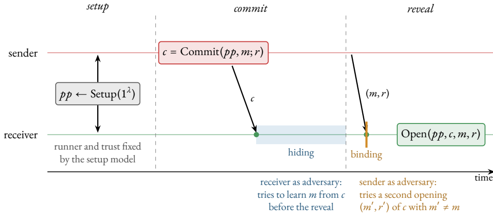
Figure 7. The three phases of Remark 4.2. In the setup phase, Setup produces the public parameters pp for both parties; who runs it, and whether that party is trusted, is fixed by the setup model (Remark 4.3). In the commit phase the sender (red), holding the secret (m, r) , transmits c = \text{Commit}(pp, m; r) and nothing else; from that point until the reveal, hiding (blue) protects the sender against a receiver who tries to learn m from c . In the reveal phase the sender transmits the opening (m, r) and the receiver (green) runs Open; at that point binding (amber) protects the receiver against a sender who could open c to a second message.
